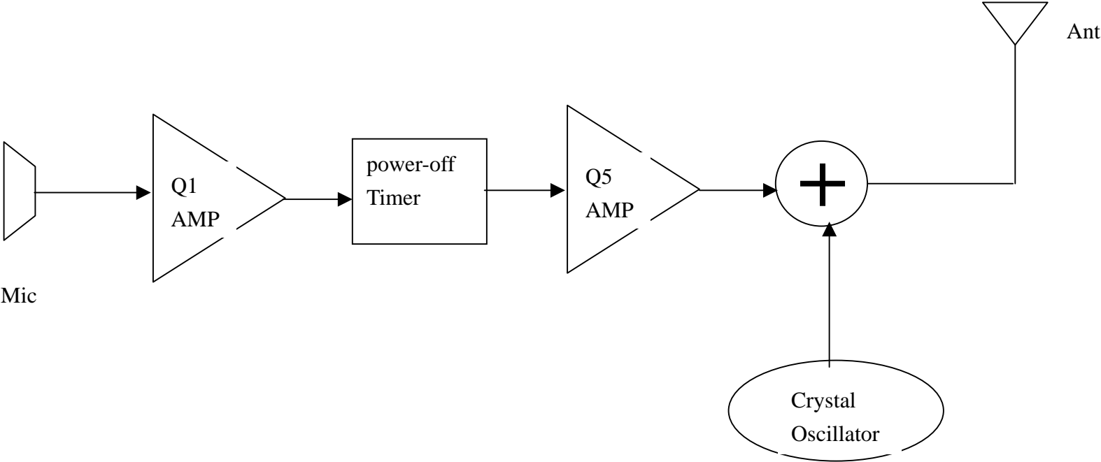
Block Diagram of HFK2MI4 microphone
