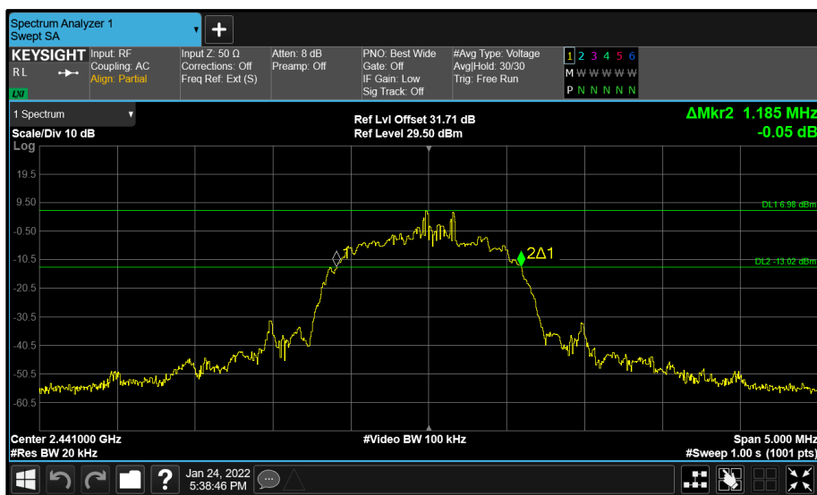
Figure 23 - R Cup (A) 2441 MHz (CH39) 20 dB Bandwidth
