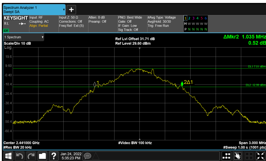
Figure 17 - R Cup (A) 2441 MHz (CH39) 20 dB Bandwidth
