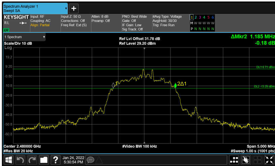
Figure 24 - R Cup (A) 2480 MHz (CH78) 20 dB Bandwidth
