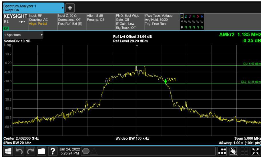
Figure 19 - R Cup (A) 2402 MHz (CH0) 20 dB Bandwidth
