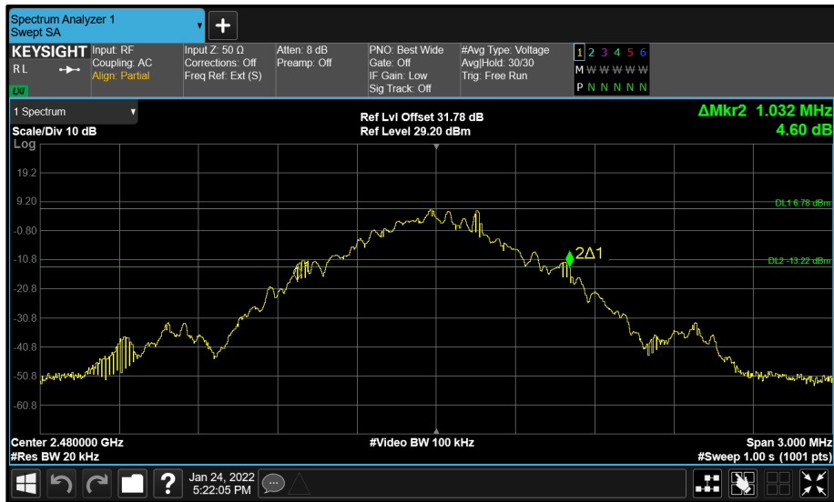
Figure 18 - R Cup (A) 2480 MHz (CH78) 20 dB Bandwidth
