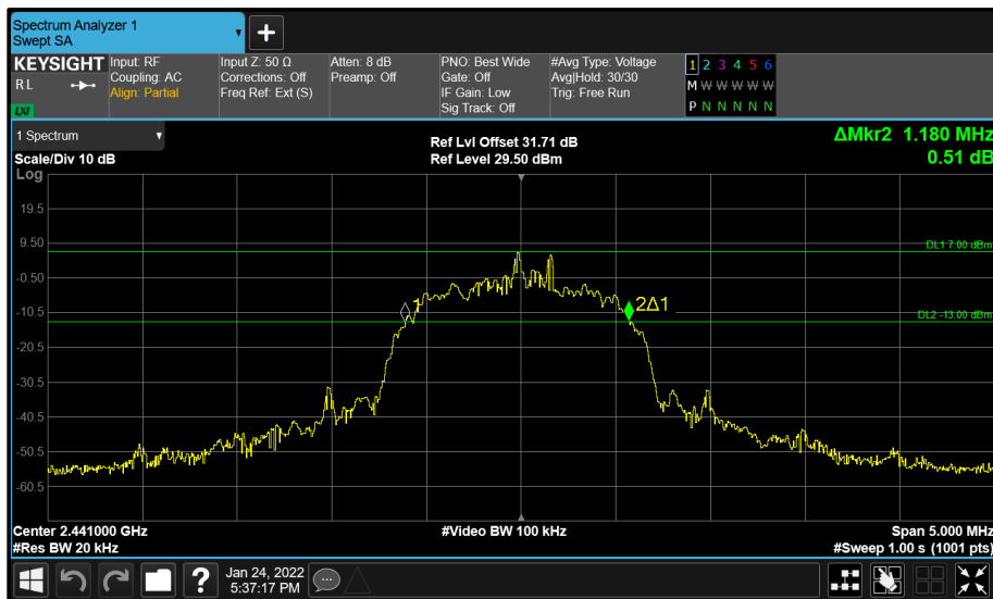
Figure 20 - R Cup (A) 2441 MHz (CH39) 20 dB Bandwidth
