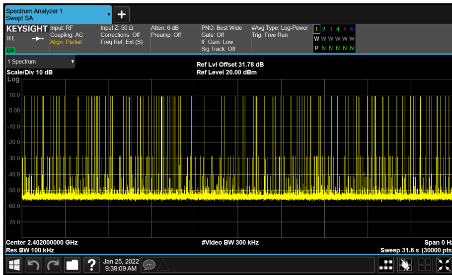
Figure 8 - GFSK - 2402 MHz Accumulated Transmit Time
