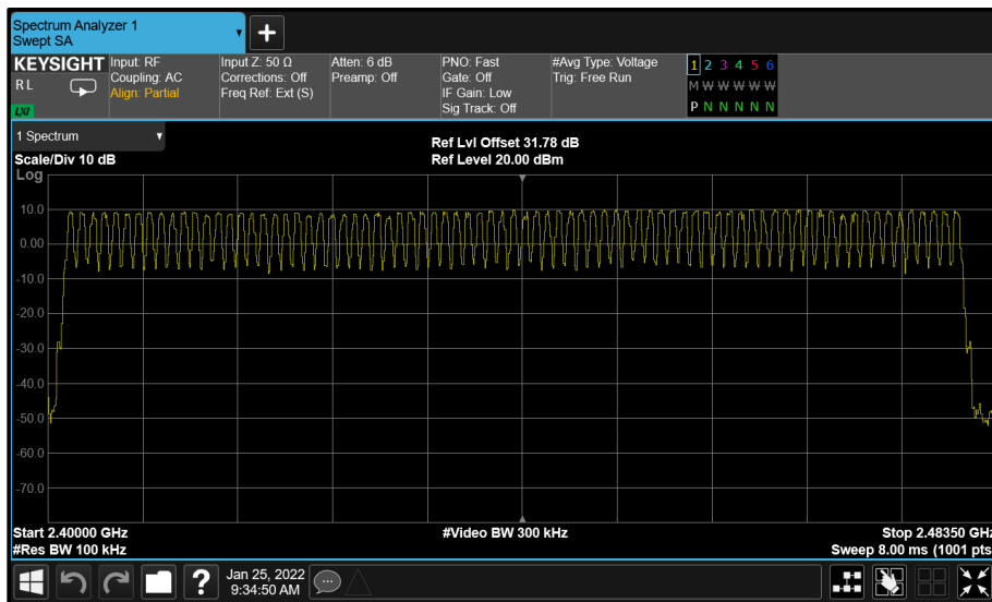
Figure 13 - GFSK (DH1) - Number of Hopping Channels
