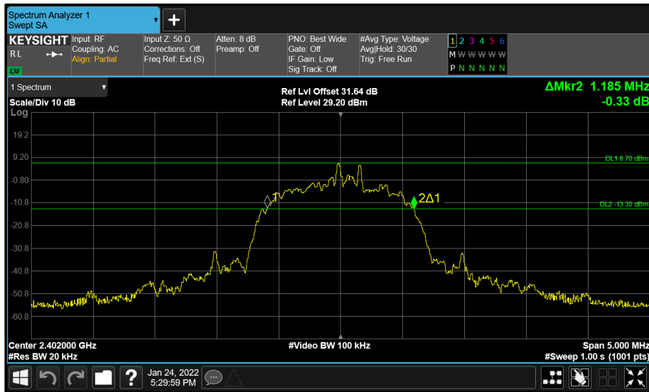
Figure 22 - R Cup (A) 2402 MHz (CH0) 20 dB Bandwidth
