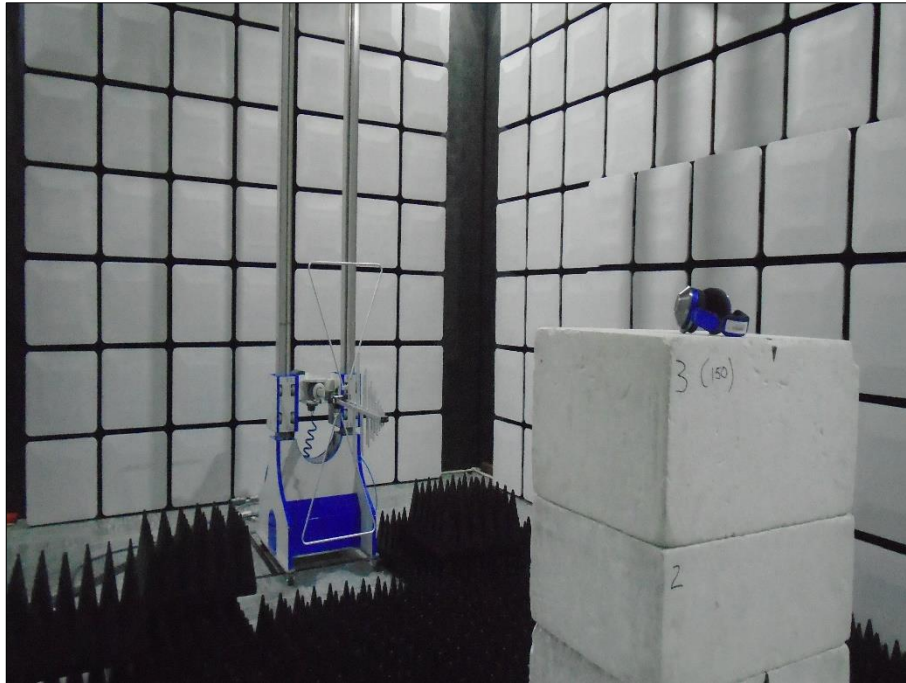
Figure 48 - Test Setup - 30 MHz to 1 GHz
