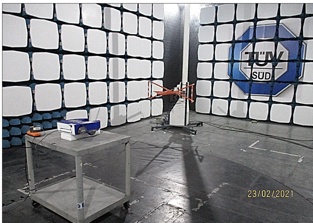
Figure 1 - Test Setup - 30 MHz to 1 GHz
