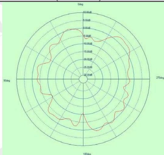
Free Space EIRP (2472MHz) - XZ cut
