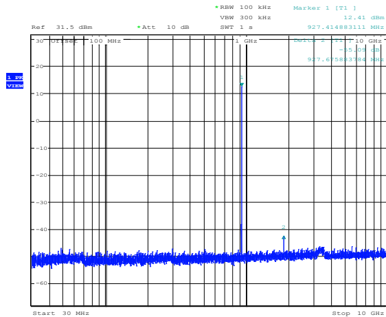
Figure 8.3-3: Conducted (TX 927 MHz)
