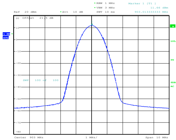
Figure 8.2-1: Conducted output power (TX 903 MHz)
