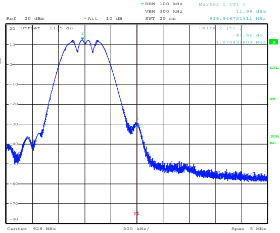
Figure 8.3-5: Upper band edge, conducted (TX 927 MHz)
