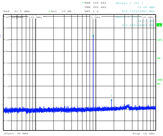
Figure 8.3-2: Conducted (TX 915 MHz)
