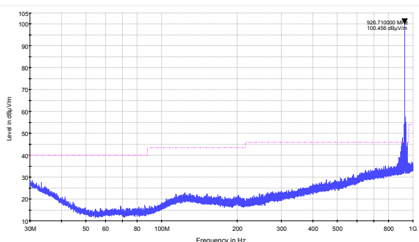
30 MHz to 1 GHz (High channel)
