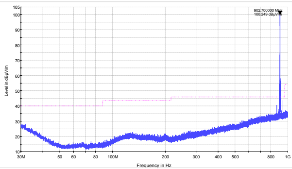
30 MHz to 1 GHz (Low channel)
