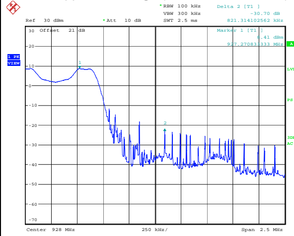
Upper band edge (Tx set to 927.3 MHz)
