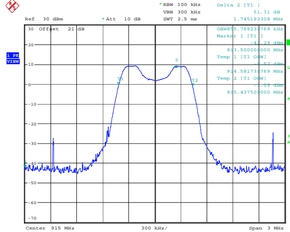
99 % occupied bandwidth
