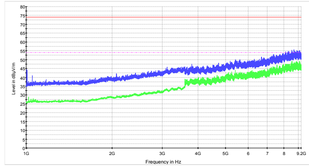
1 GHz to 9.2 GHz (Low channel)
