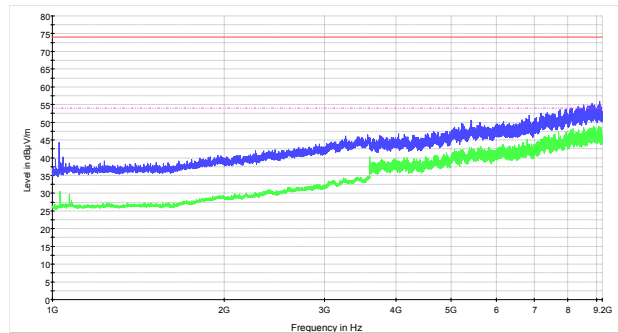
1 GHz to 9.2 GHz (Mid channel)
