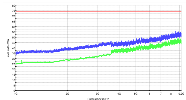
1 GHz to 9.2 GHz (High channel)
