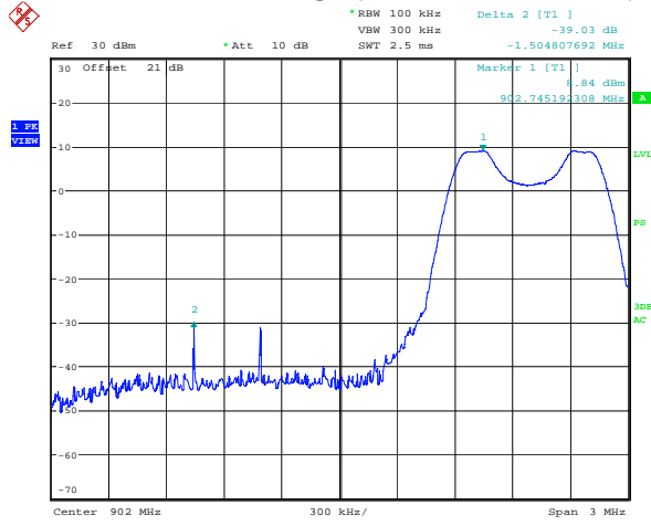
Lower band edge (Tx set to 902.7 MHz)
