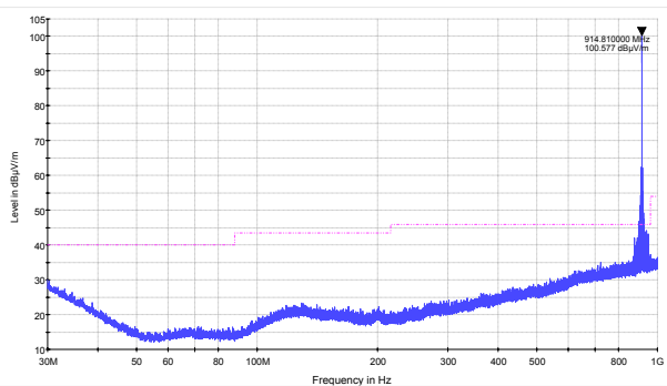
30 MHz to 1 GHz (Mid channel)
