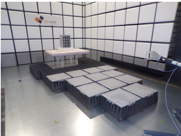
Test setup for frequency above 1GHz
