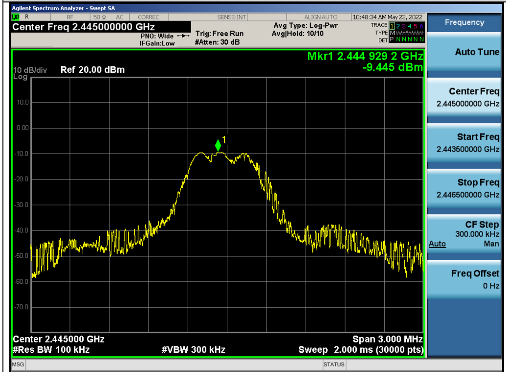
Test_Graph_GFSK_ANT1_2445_Reference Level
