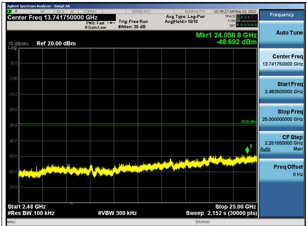
Test_Graph_GFSK_ANT1_2409_Higher Band Emissions
