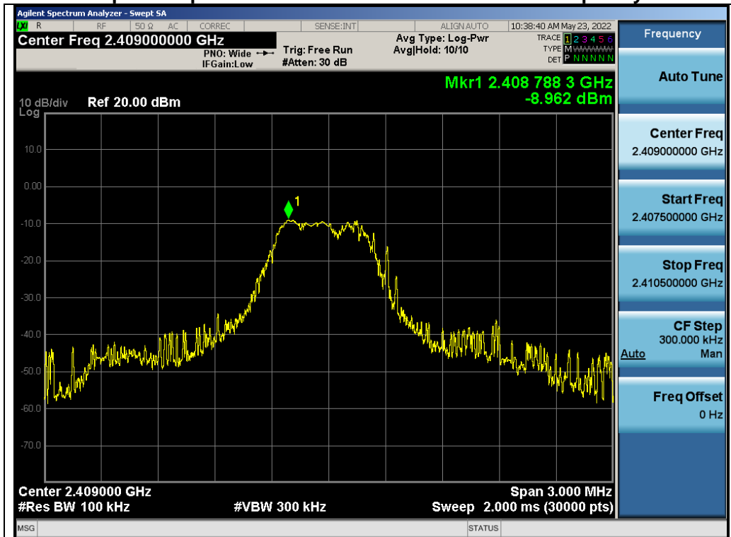
Test_Graph_GFSK_ANT1_2409_Reference Level
