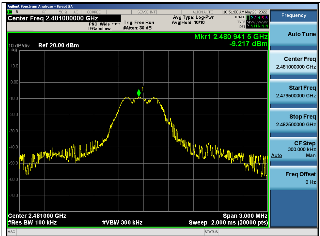
Test_Graph_GFSK_ANT1_2481_Reference Level
