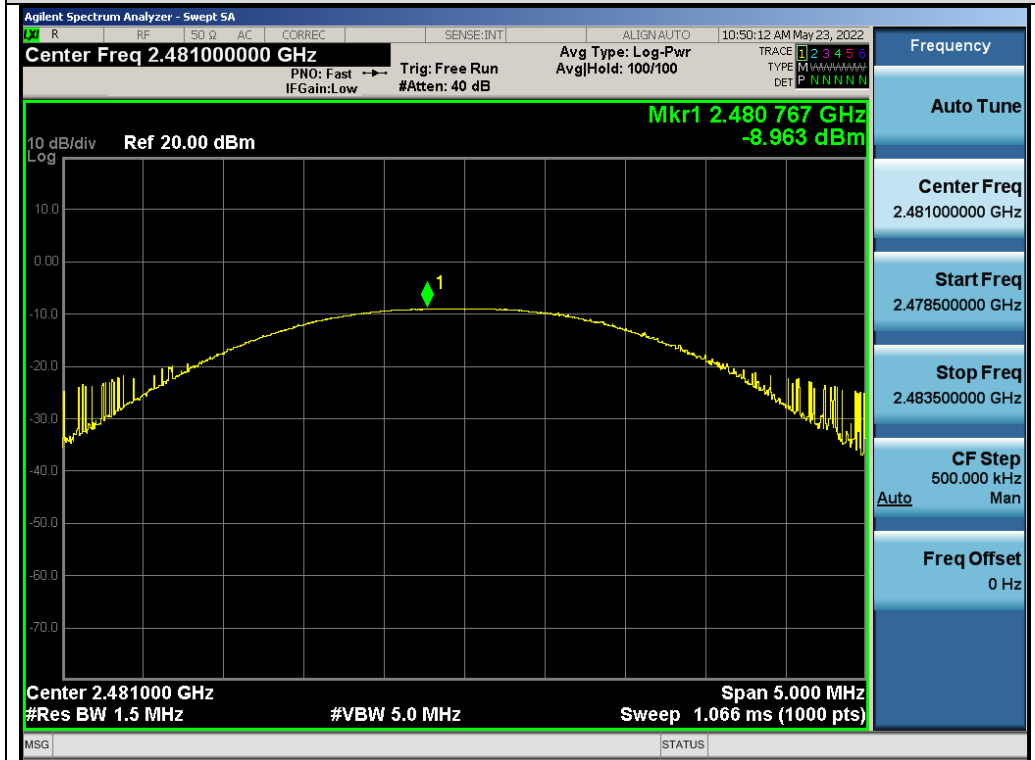
Test_Graph_GFSK_ANT1_2481_Peak Power
