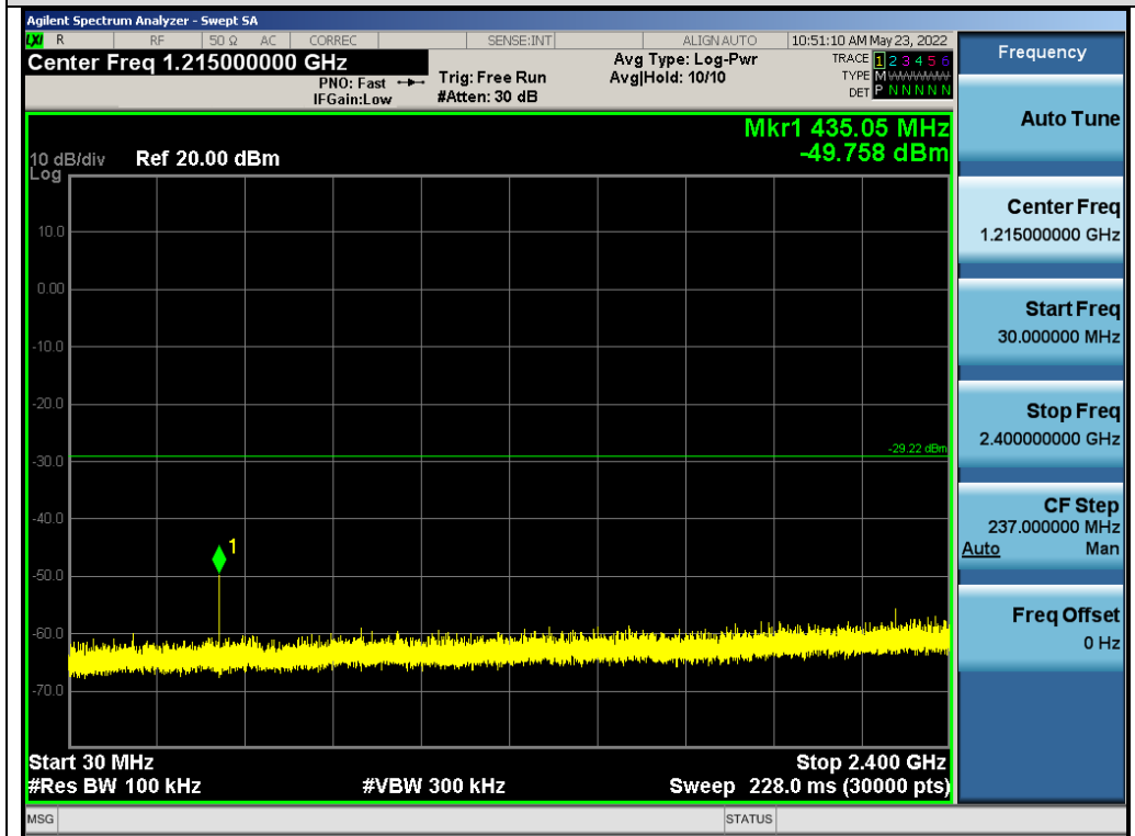
Test_Graph_GFSK_ANT1_2481_Lower Band Emissions
