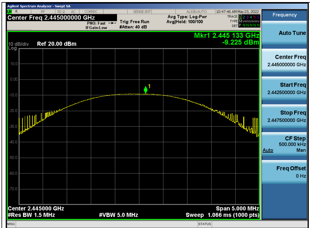
Test_Graph_GFSK_ANT1_2445_Peak Power
