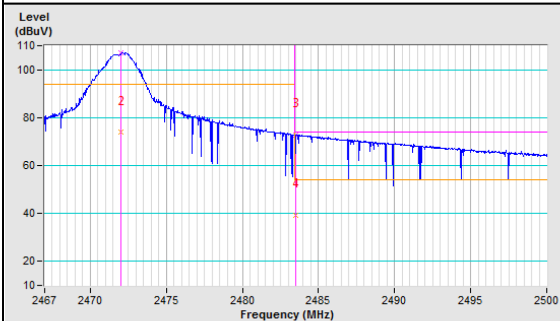
2472MHz Vertical
