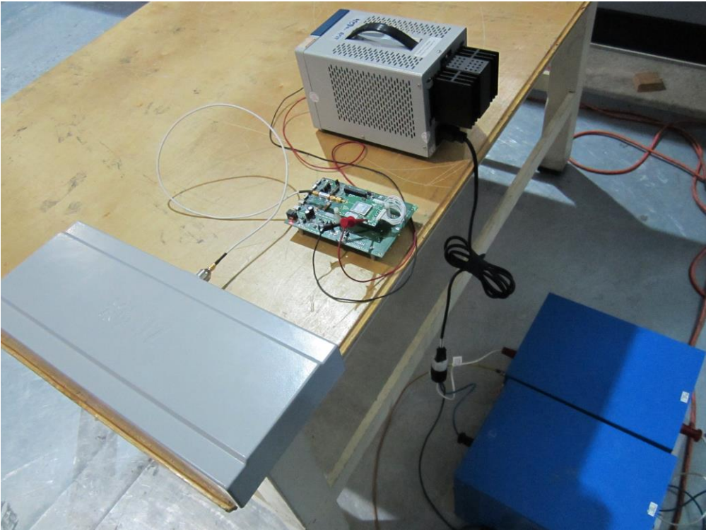
CEMI Radiated - Rear
