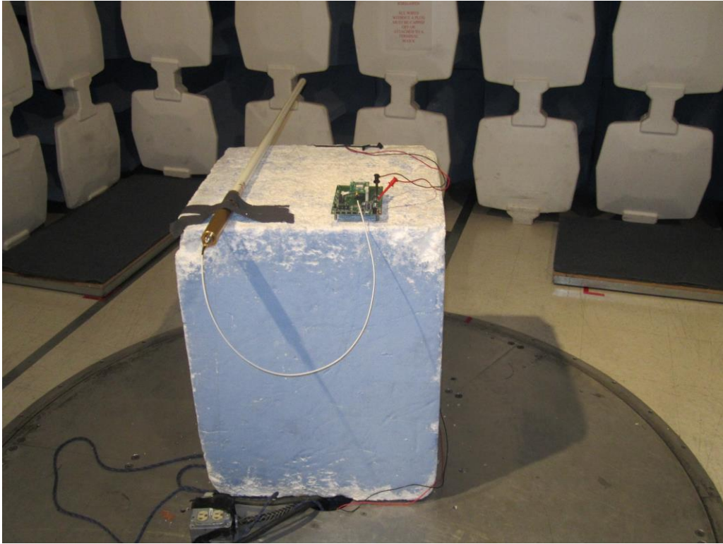
EMI Radiated – Closed up View
