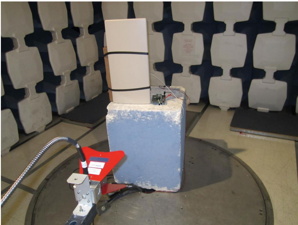
EMI Radiated – 6-10GHz
