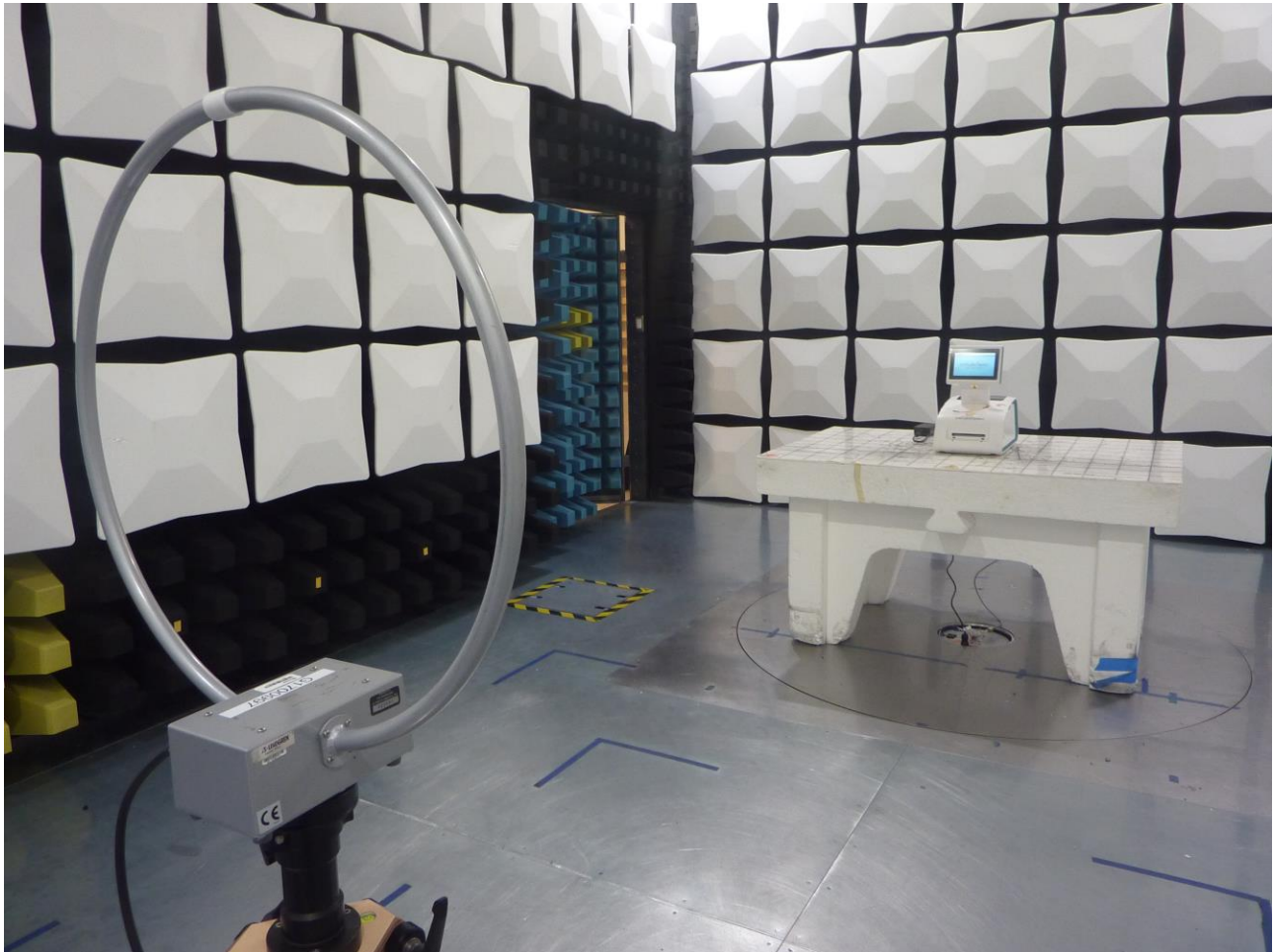
Figure 1: Test Setup for Radiated Emissions 9 kHz to 30 MHz
