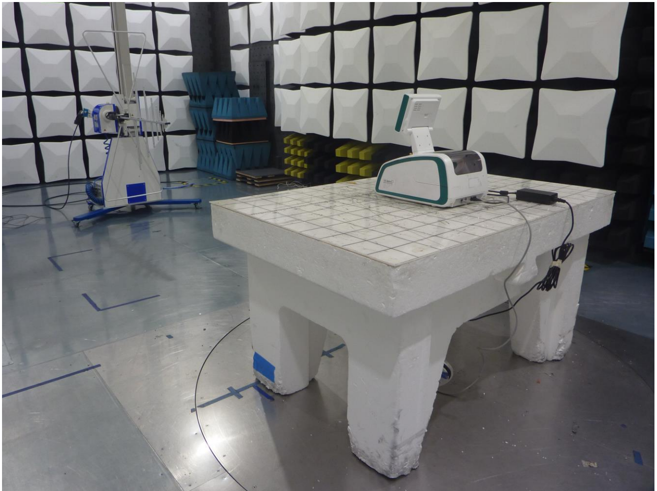
Figure 2: Test Setup for Radiated Emissions 30 MHz to 1000 MHz
