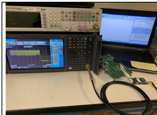
Conducted test setup
