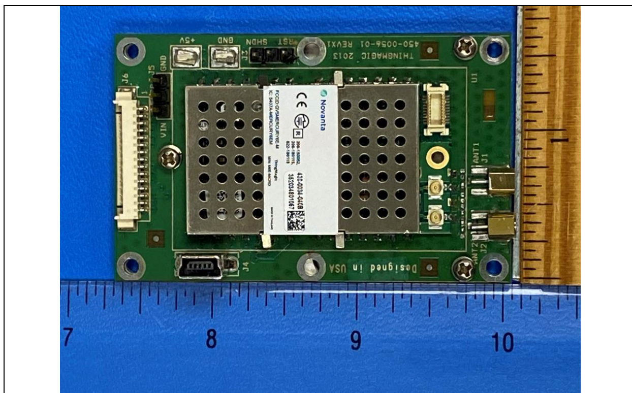
RF module soldered to Carrier board top with shielding view
