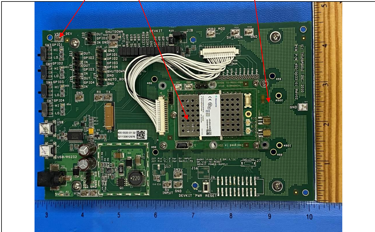
EUT soldered to carrier board with M6E-DEVKIT Top View
