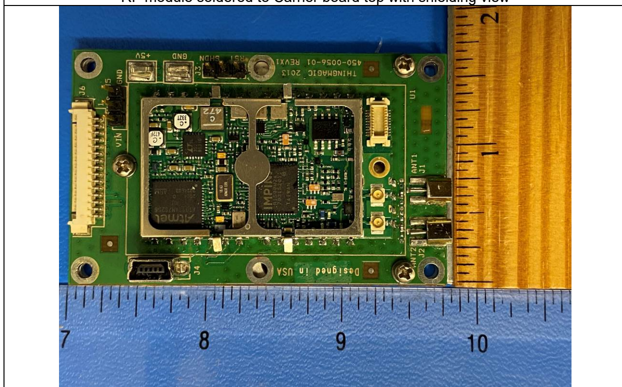
RF module soldered to Carrier board top without shielding view
