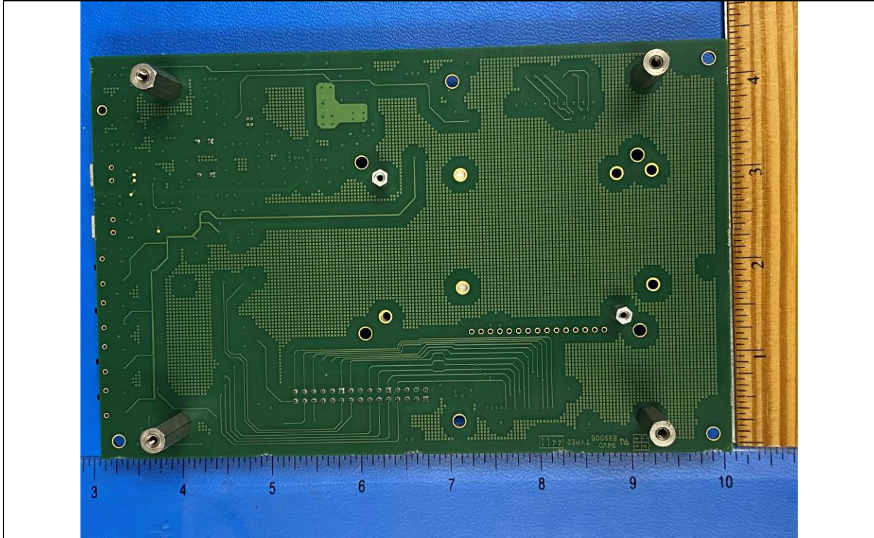
M6e-DEVKIT Bottom View
