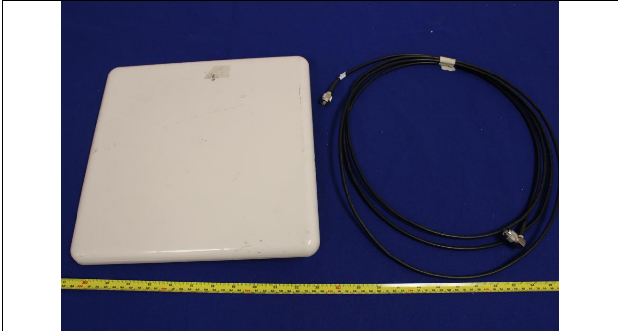
RHCP Patch Antenna top view with cable
