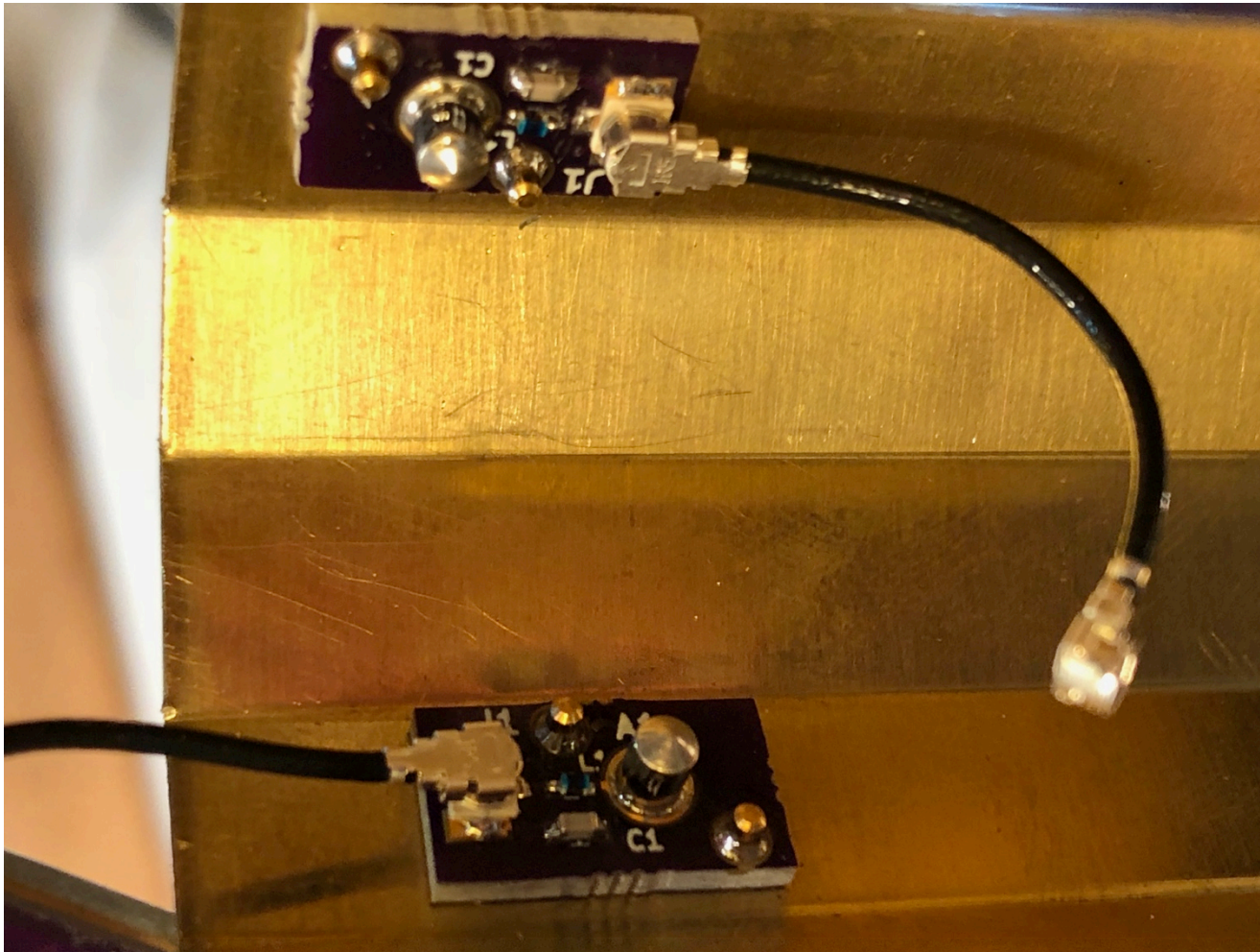
ADASA DLP915A1 Internal Photos
