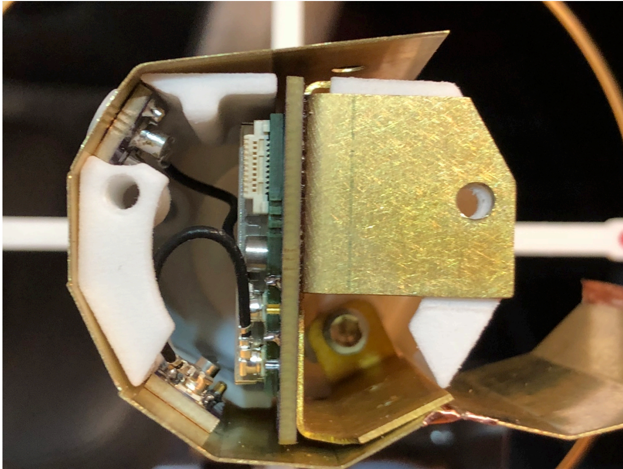
ADASA DLP915A1 Internal Photos
