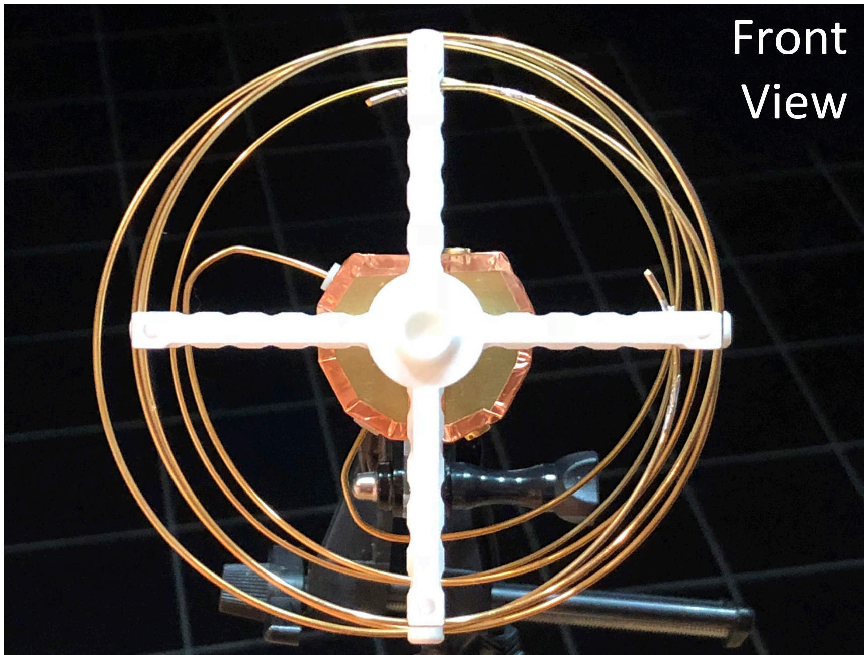
ADASA DLP915A1 External Photos
