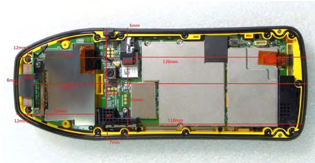
Fig.11 Antenna position of EUT
