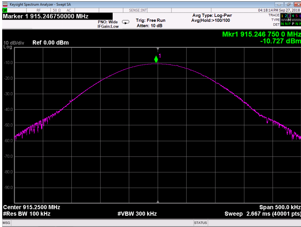
Port 2 Mid
