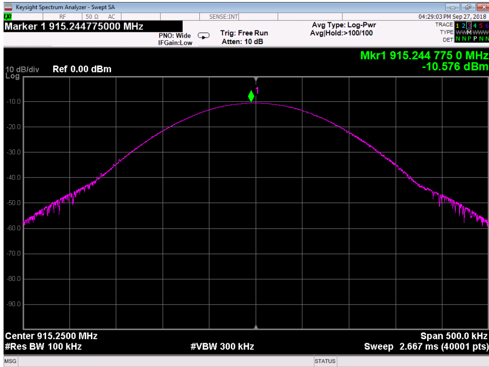
Port 4 Mid
