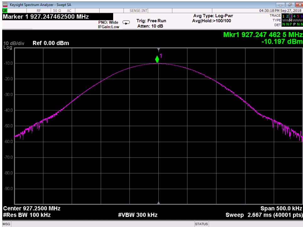
Port 4 High
