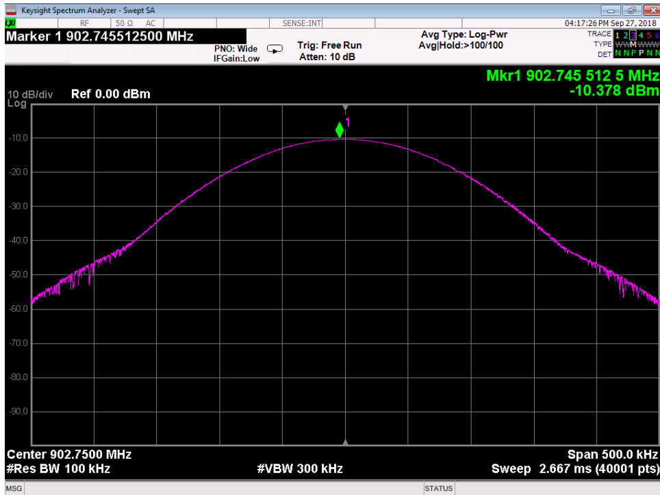
Port 2 Low
