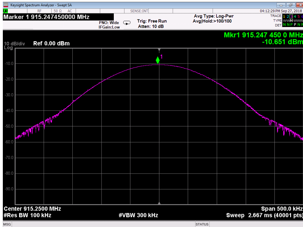
Port 1 Mid
