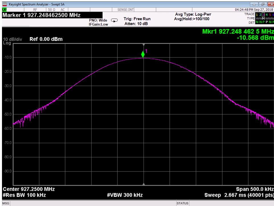
Port 2 High
