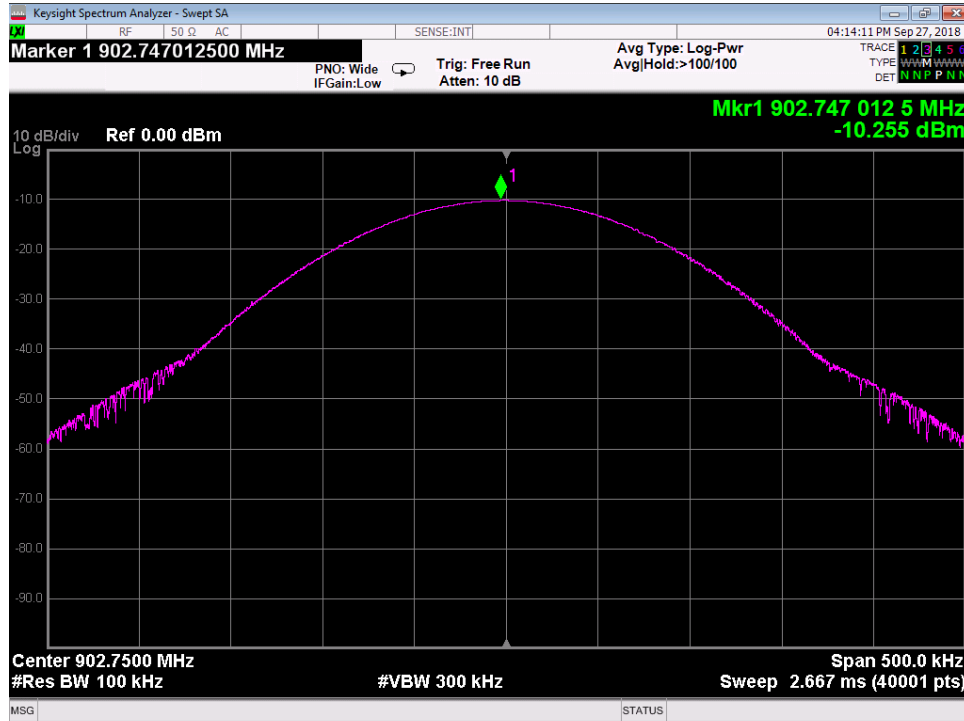
Port 1 Low
