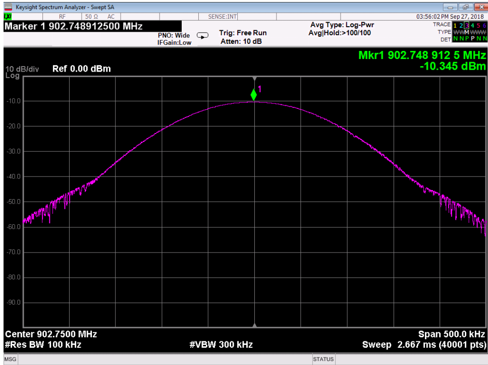
Port 3 Low
