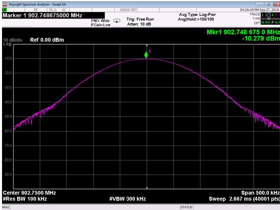
Port 4 Low
