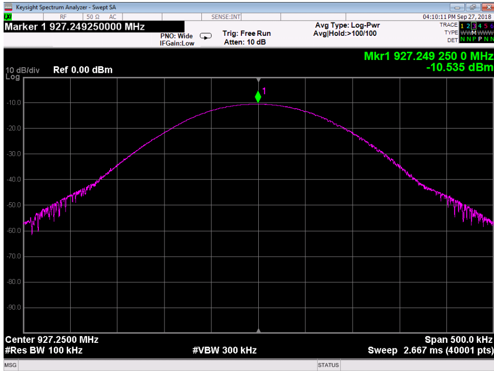
Port 1 High
