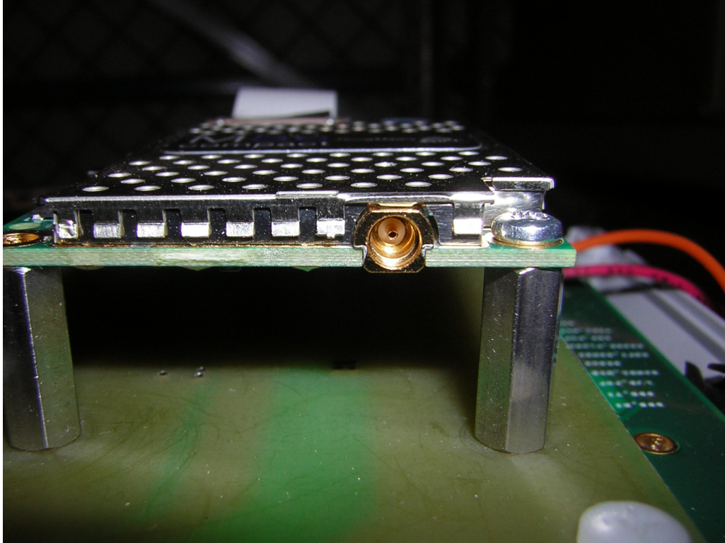
M5e-Compact Antenna connector – Female (jack) MMCX
