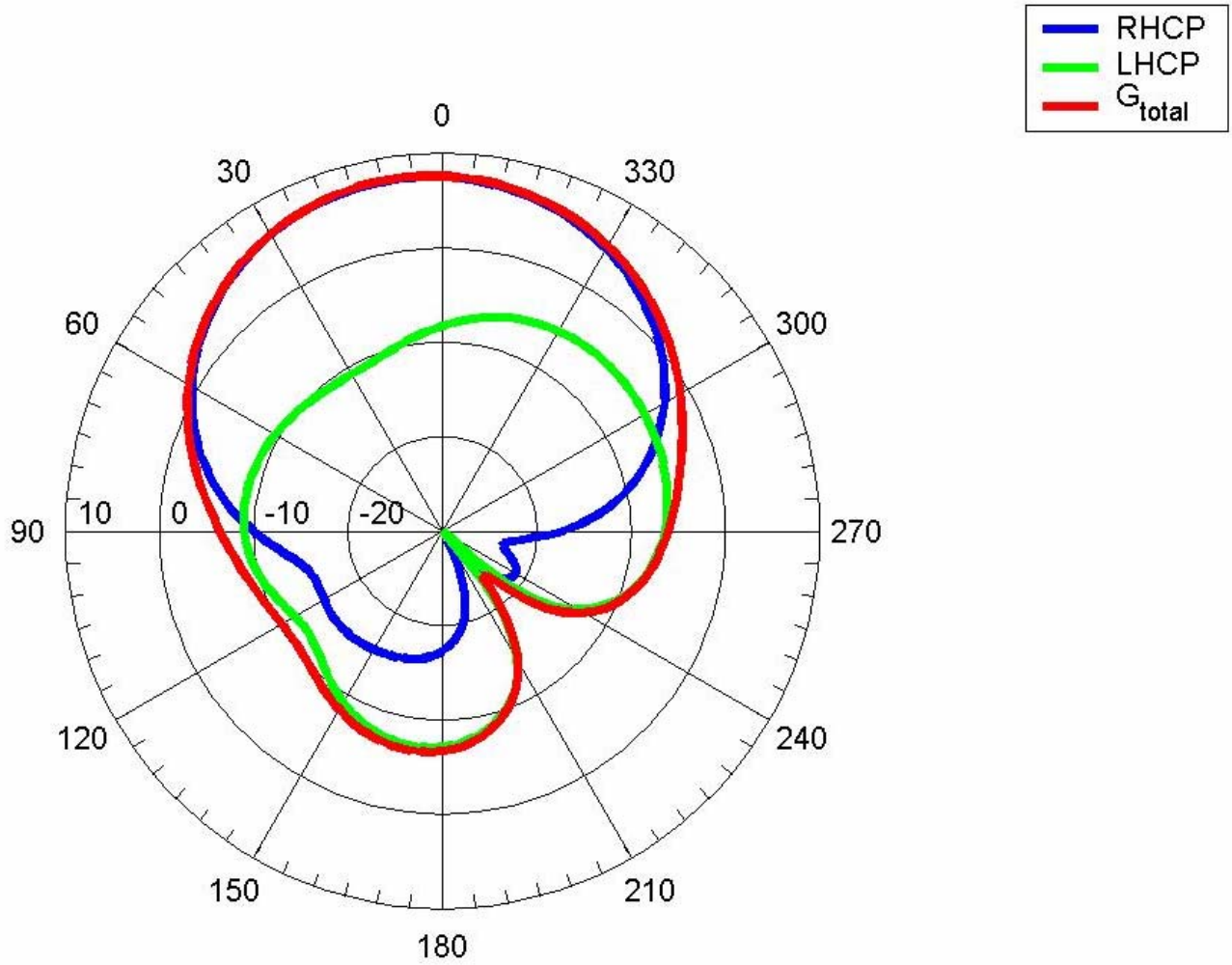
Azimuth Plot vs \phi , x-y plane, \theta = 90
