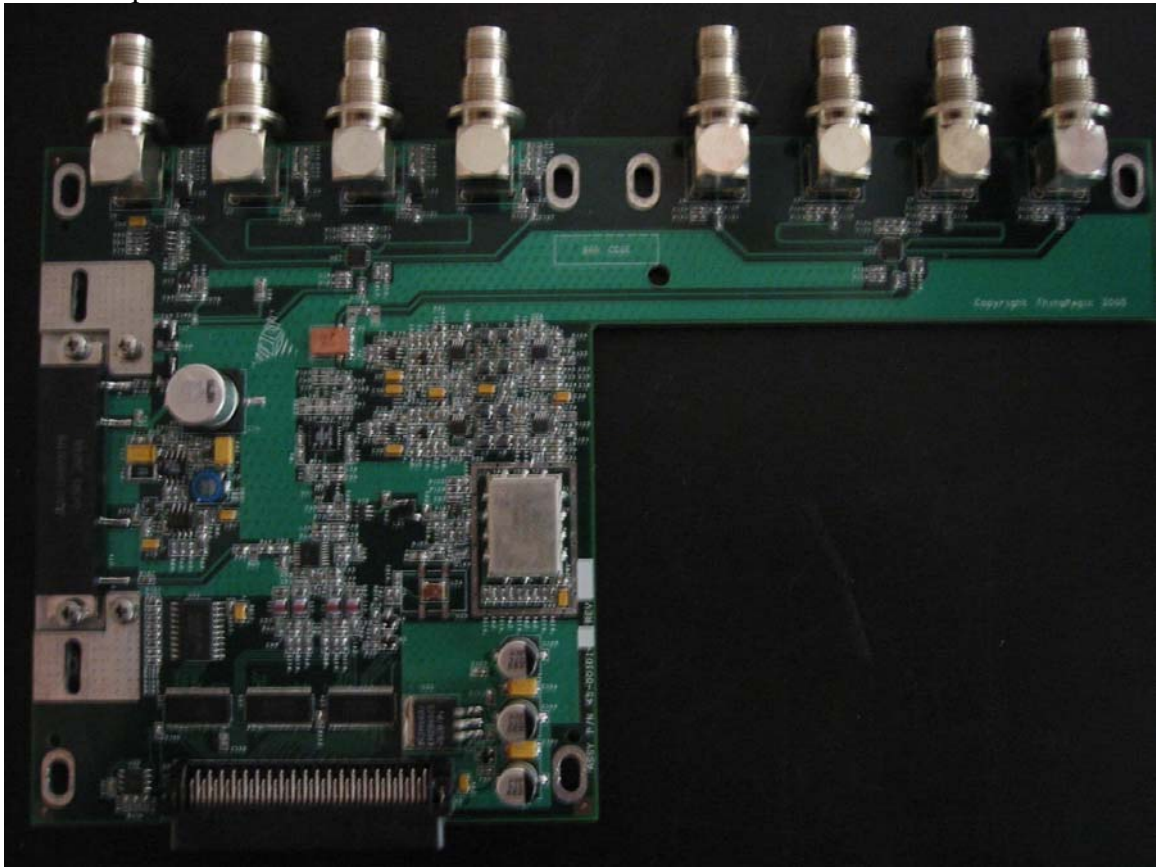
PCB 1 Top
