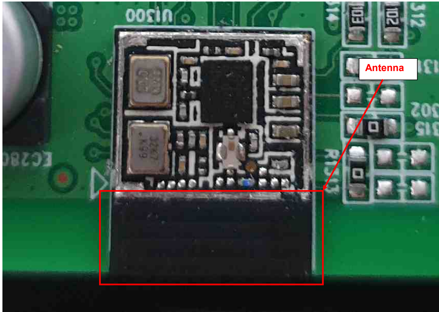
[Bluetooth Module]
