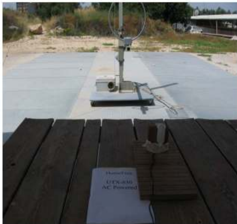
Figure 4. Radiated Emission Test 9 kHz – 30 MHz
