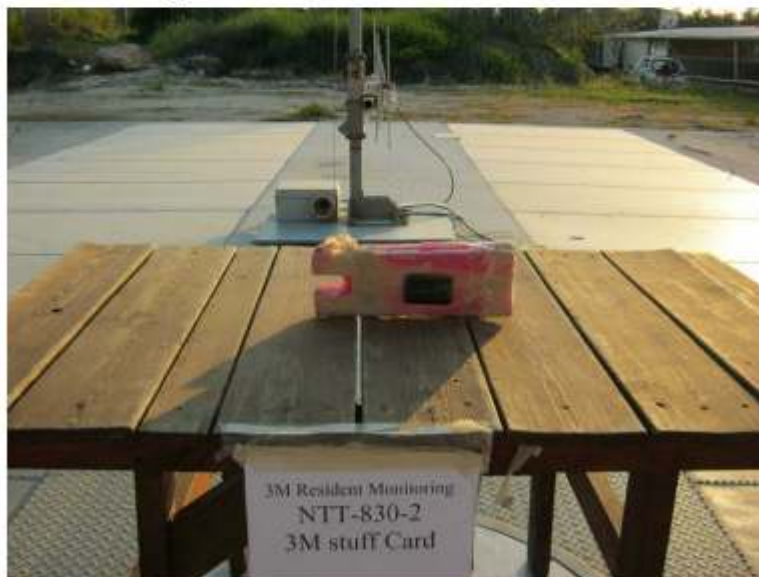
Figure 3. Radiated Emission Test 30 MHz – 4500MHz
