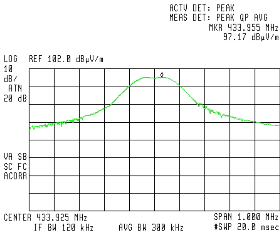
Figure 12. Field Strength of Fundamental. Antenna Polarization: VERTICAL.
