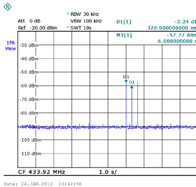
Figure 5. Time Between Bursts > 100 ms (320msec)
