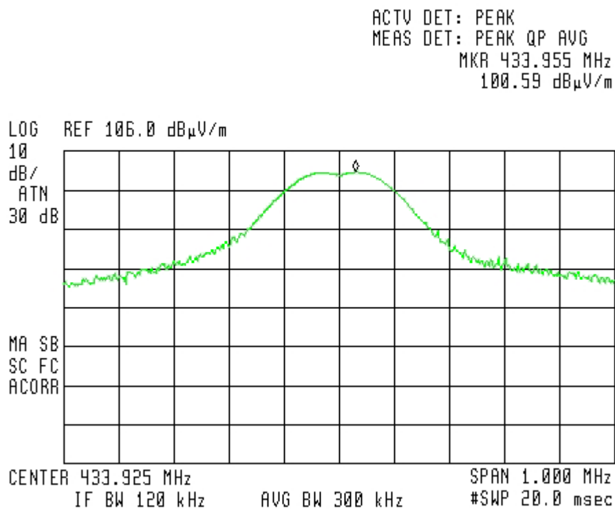
Figure 11. Field Strength of Fundamental. Antenna Polarization: HORIZONTAL.
