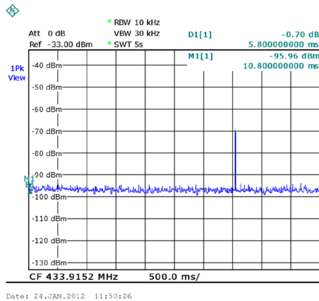
Figure 7. Automatic Transmission With Movement Detector Within 5sec
