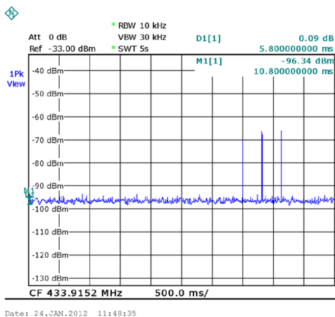
Figure 6. ON /OFF Manual Initializing Transmission
