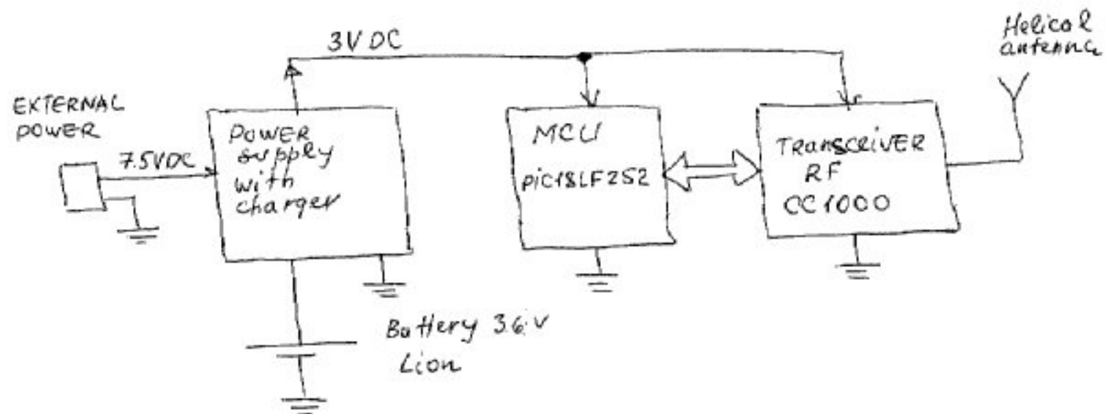
iDEU block diagram
