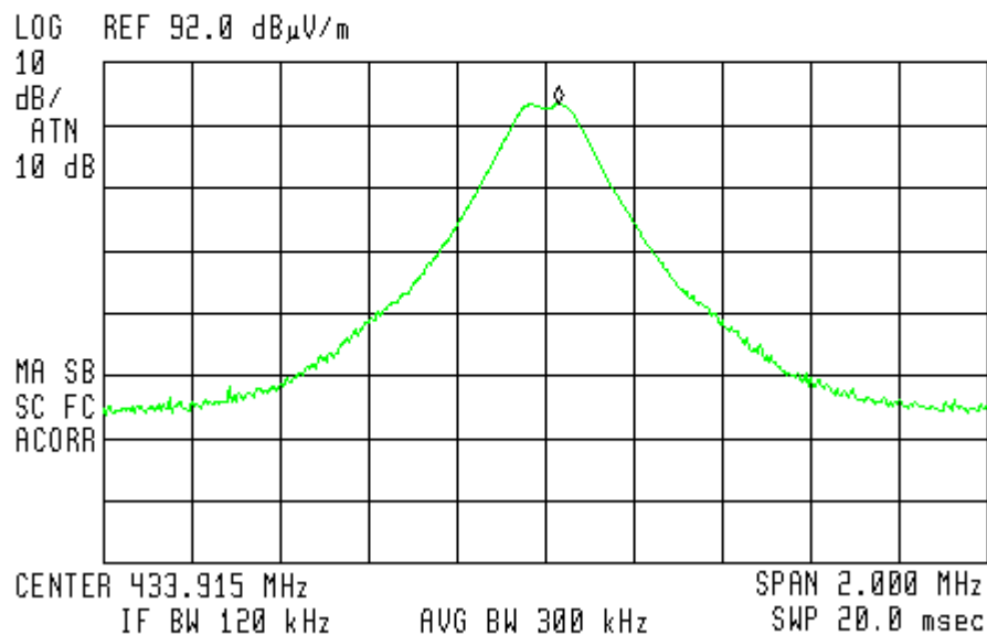
Figure 13. Field Strength of Fundamental. Antenna Polarization: VERTICAL.
