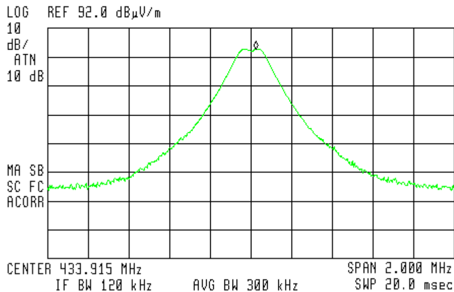
Figure 12. Field Strength of Fundamental. Antenna Polarization: HORIZONTAL.
