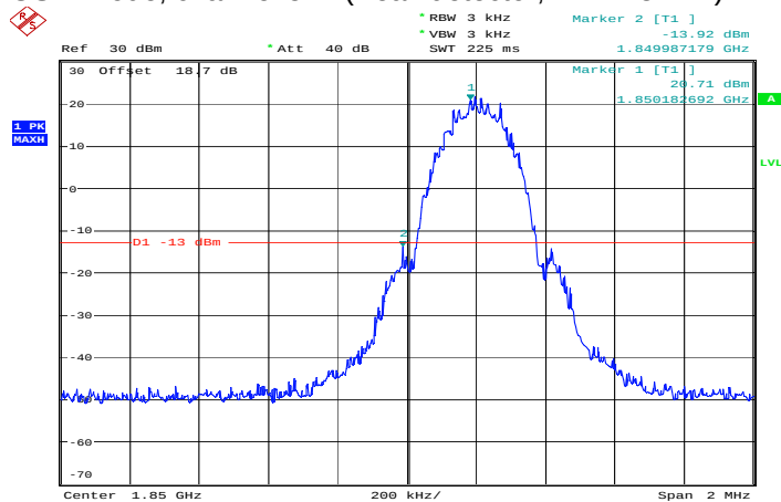
GSM mode, channel 512 (Peak detector, RBW: 3 kHz)
