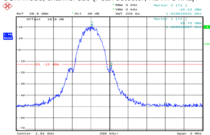
GSM mode, channel 810 (Peak detector, RBW: 3 kHz)
