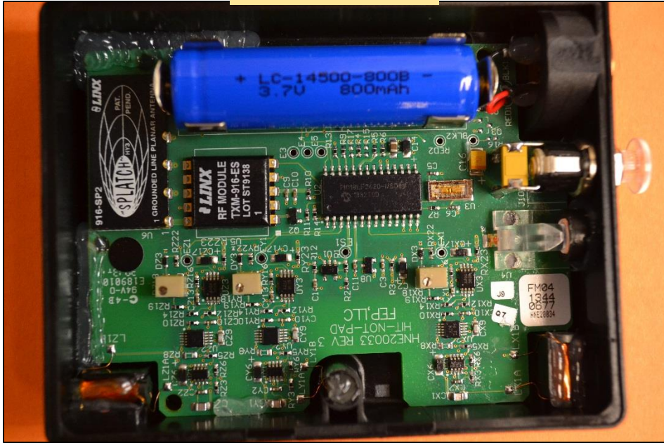
Printed Circuit Board-Top Side
