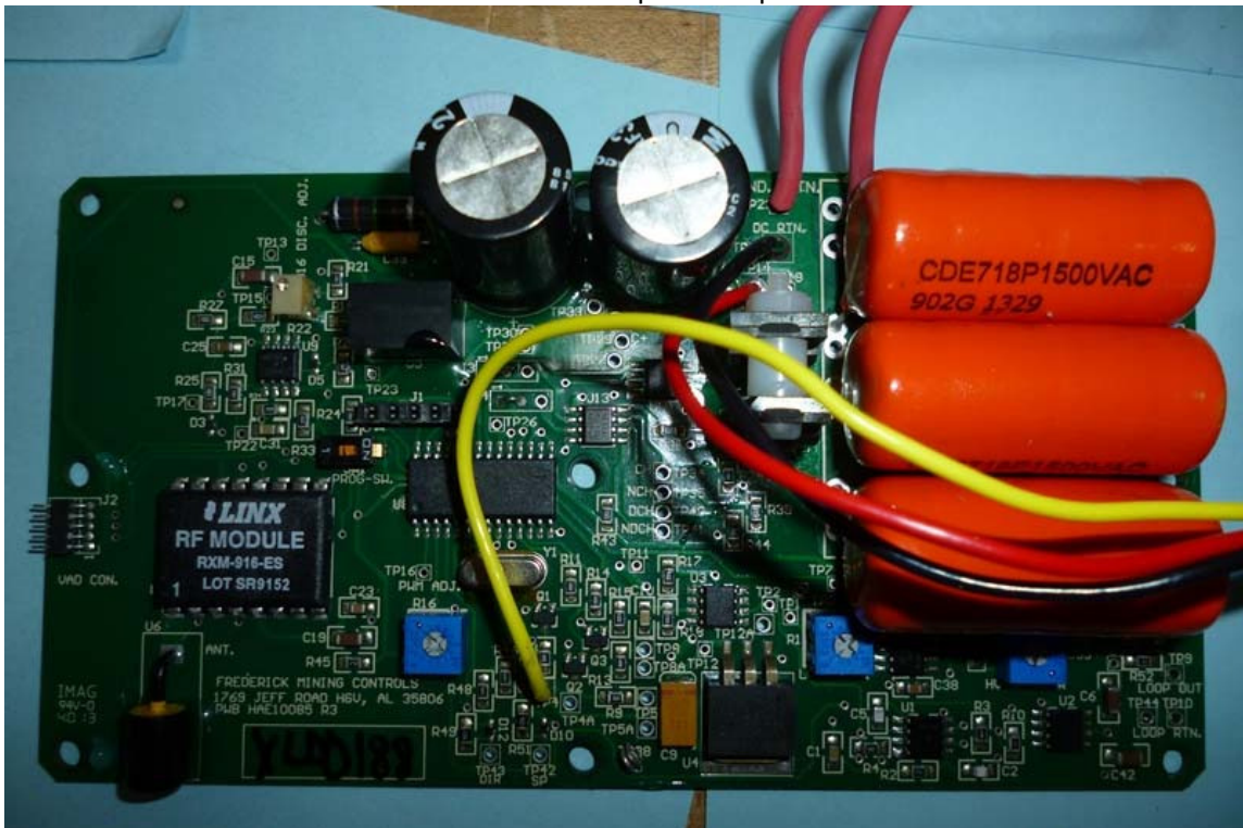
Board 2 - Top Close Up
