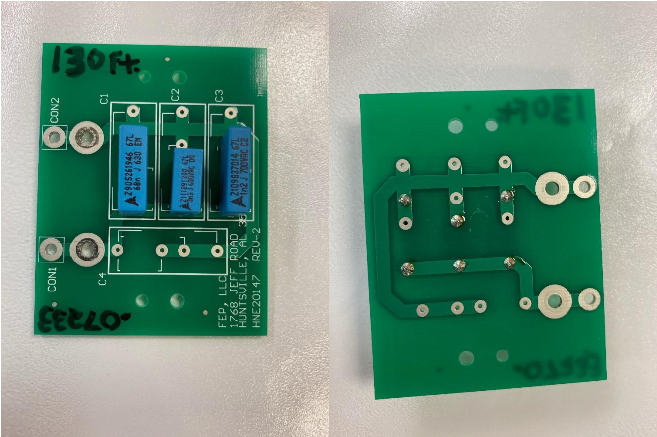
Capacitor Board- Top Side
