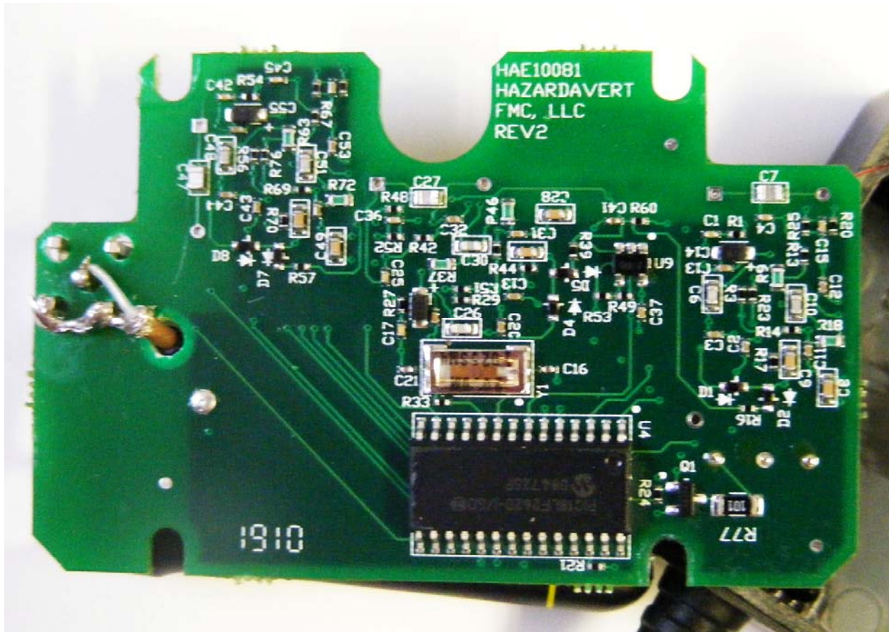
Surface Pad – Internal Photo Printed Circuit Board – Bottom Side
