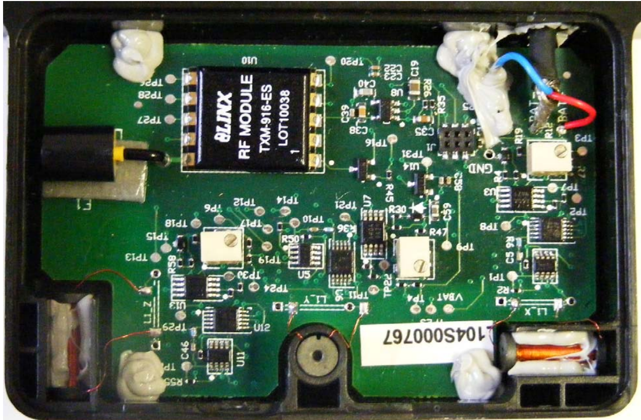
Surface Pad – Internal Photo Printed Circuit Board – Top Side
