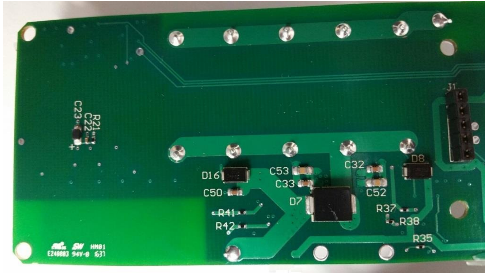
Magnetic Field Generator-Internal Photo Generator/Receiver Board-Bottom View (pt. 1)
