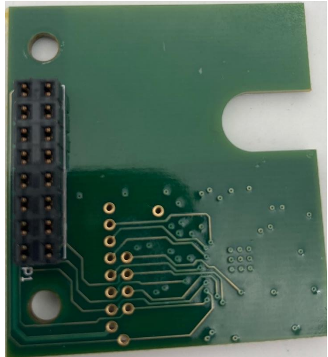
Printed Circuit Board-Back Side RF Board
