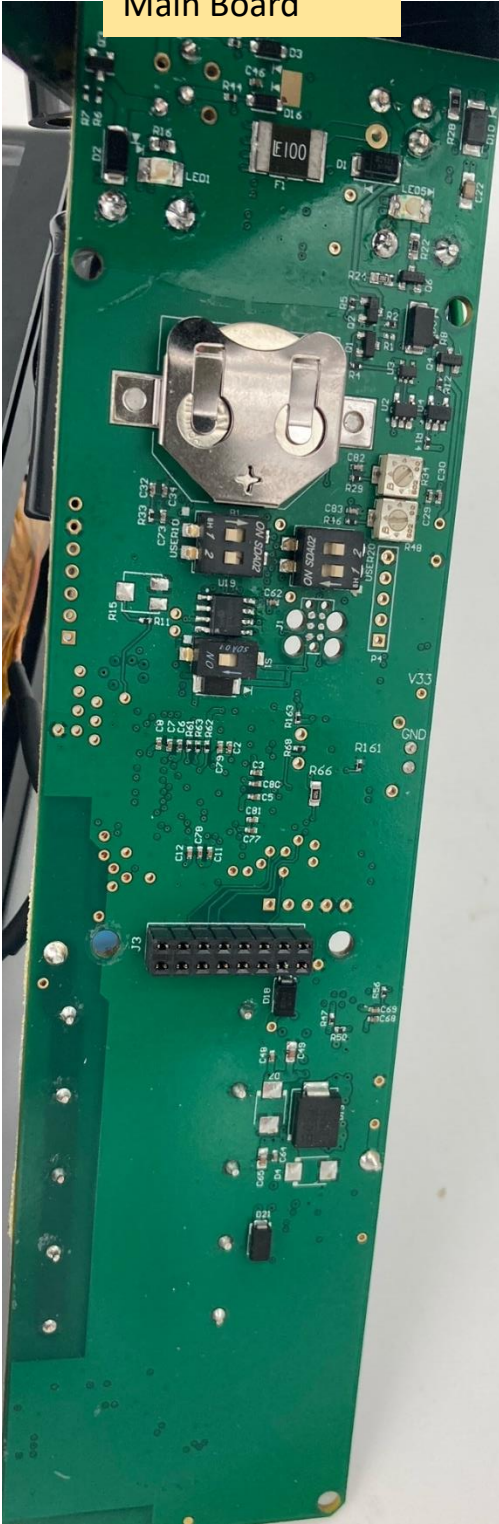
Printed Circuit Board-Top Side Main Board
