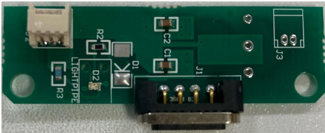
Charger Board- Top Side
