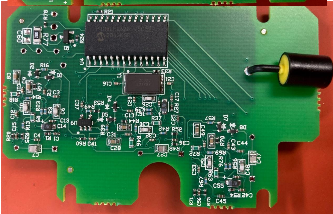
Printed Circuit Board-Back Side
