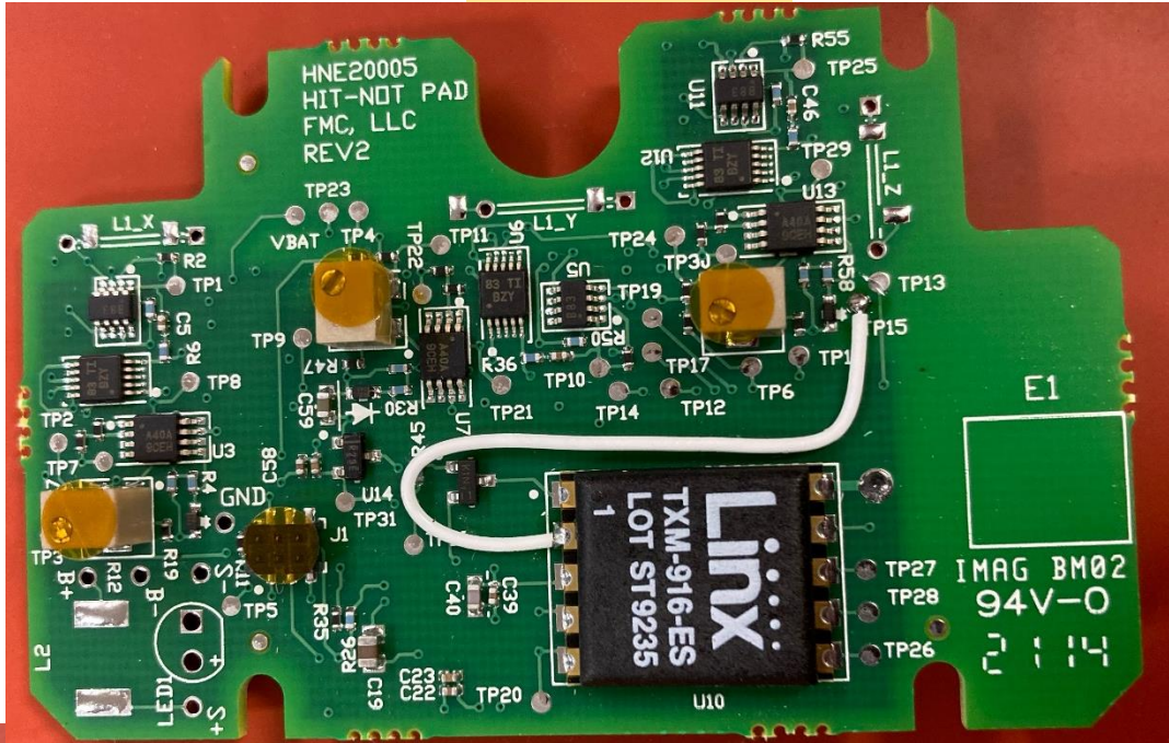
Printed Circuit Board-Top Side
