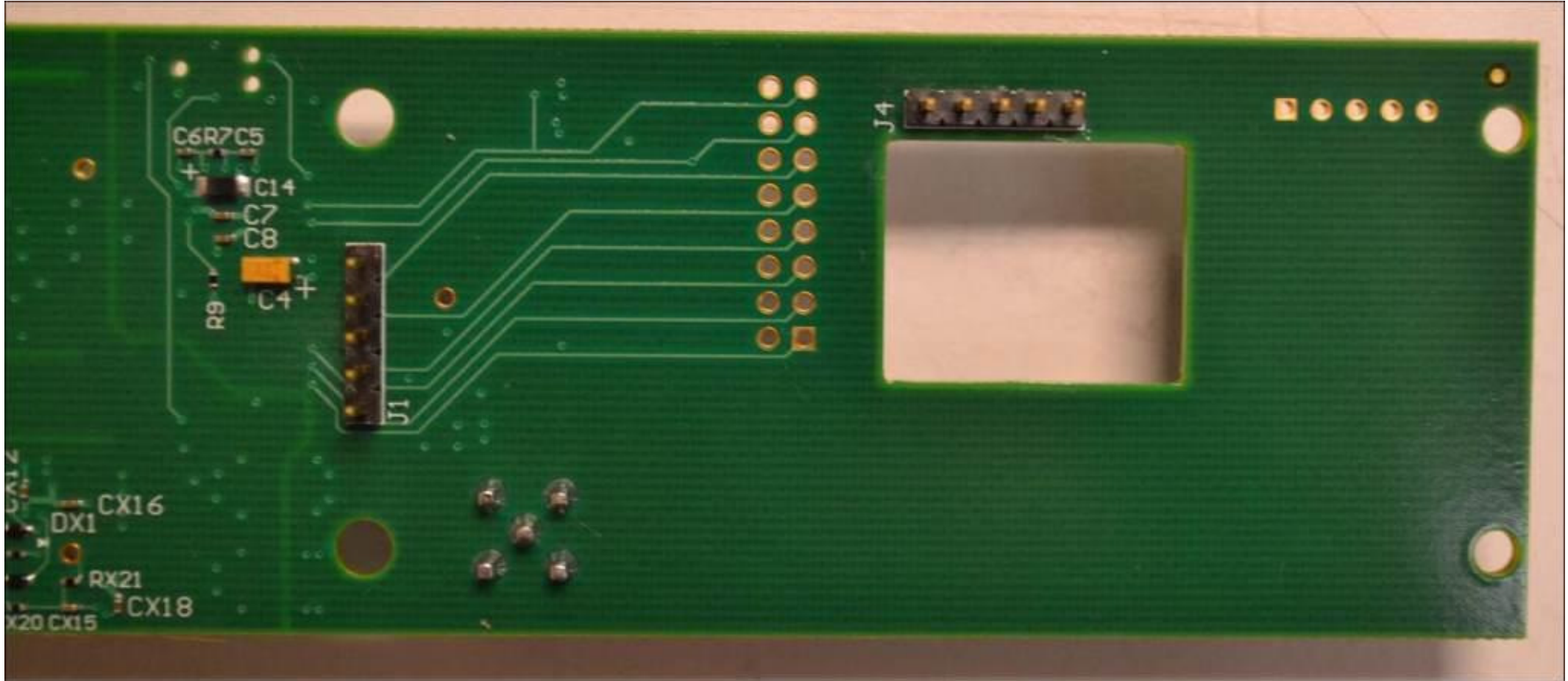
Magnetic Field Generator w/ CAM -Internal Photo CAM Board-Bottom View (pt. 2-no spacer)
