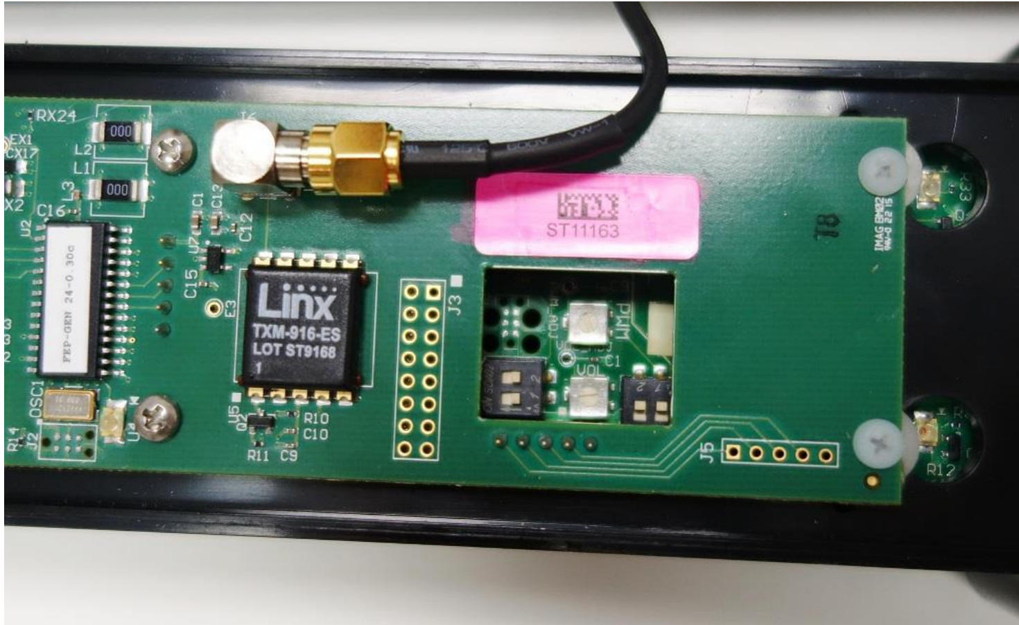
Magnetic Field Generator w/ CAM-Internal Photos Open Middle Housing Collision Avoidance Module Board (pt. 1)
