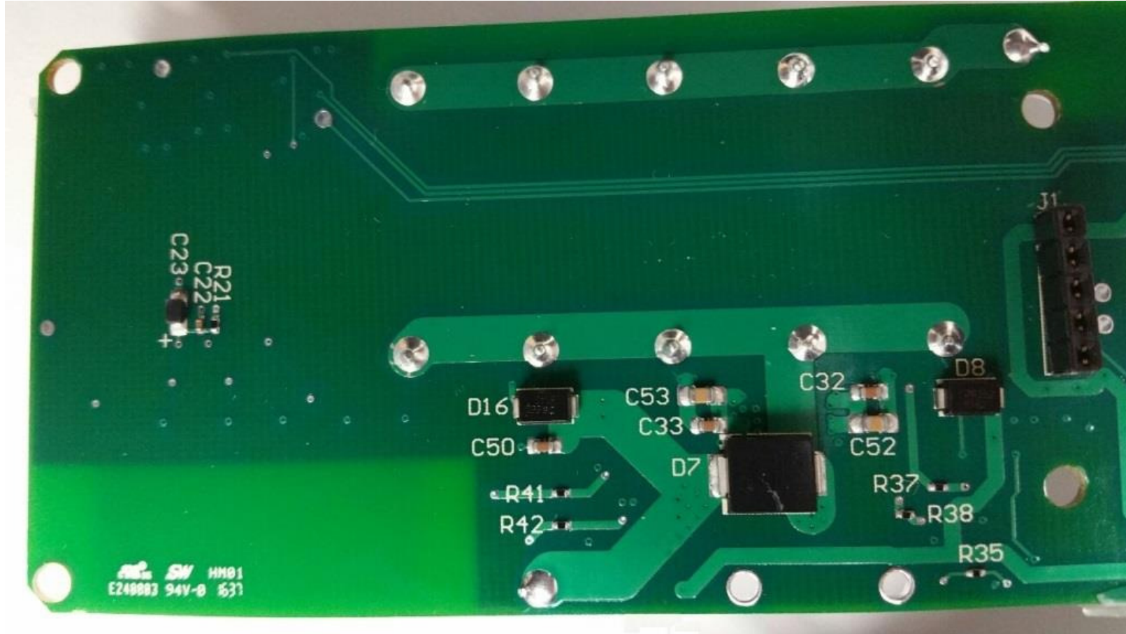
Magnetic Field Generator w/ CAM -Internal Photo Generator/Receiver Board-Bottom View (pt. 1)
