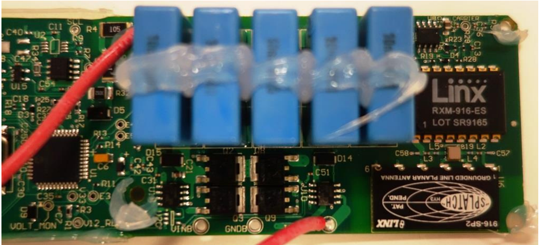
Magnetic Field Generator w/ CAM -Internal Photo Generator/Receiver Board-Top View (pt. 1)
