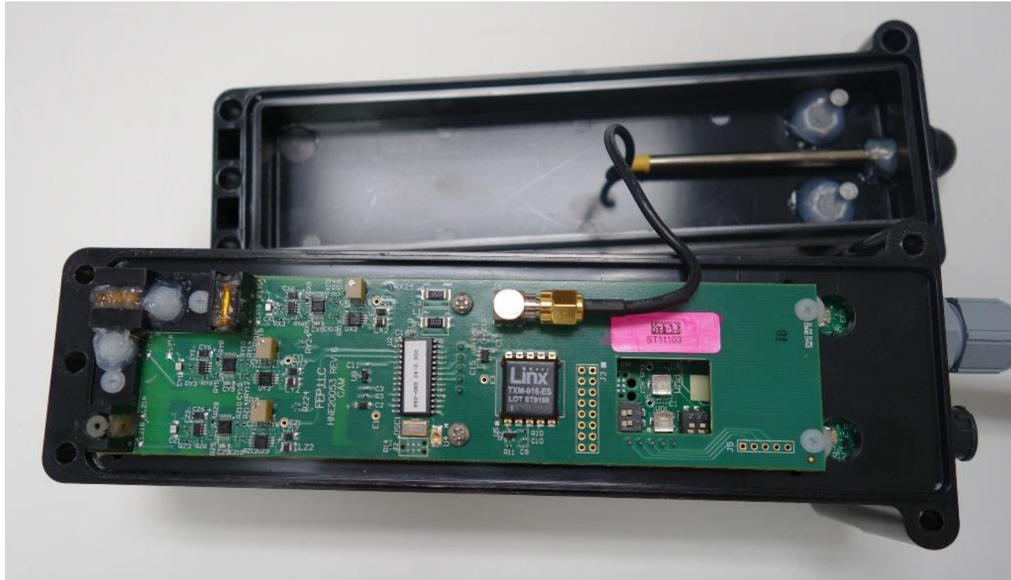
Magnetic Field Generator w/ CAM -Internal Photo Open Label and Middle Housings Circuitry and Wire/Ferrite Radiator
