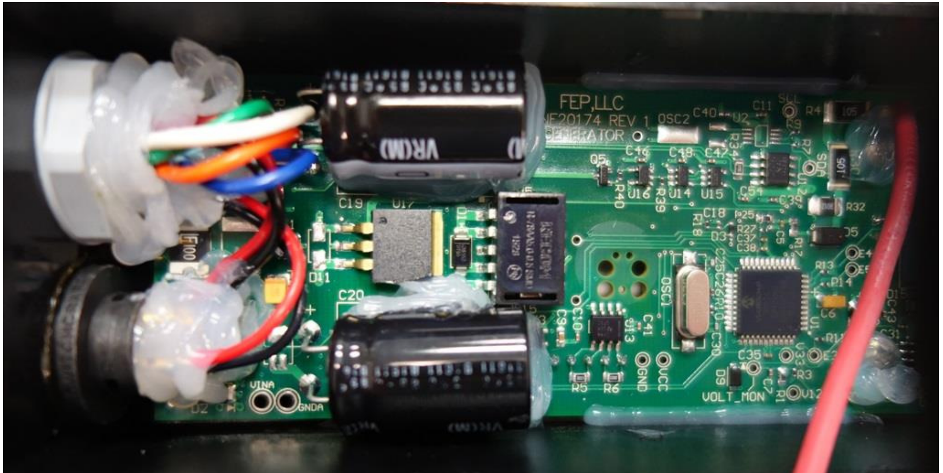
Magnetic Field Generator w/ CAM -Internal Photo Generator/Receiver Board-Top View (pt. 2)
