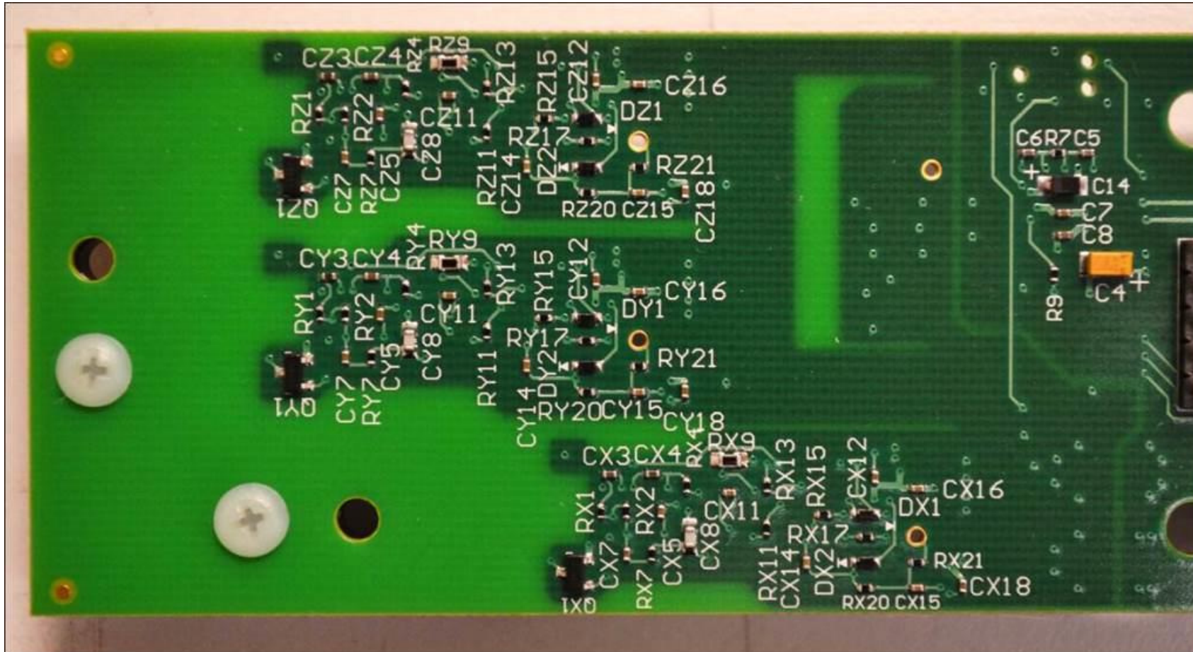
Magnetic Field Generator w/ CAM -Internal Photo CAM Board-Bottom View (pt. 1-no spacer)
