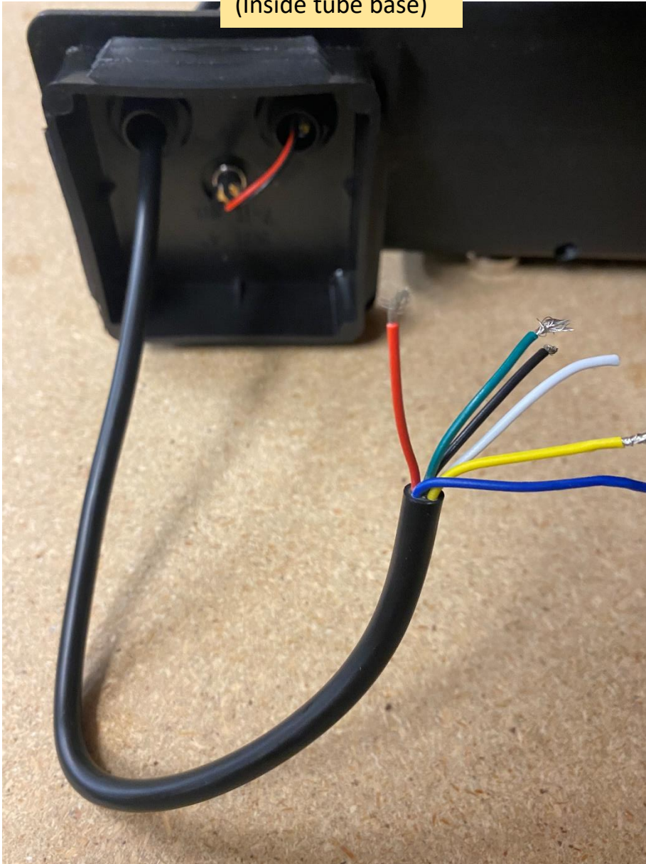
Output cable (Inside tube base)
