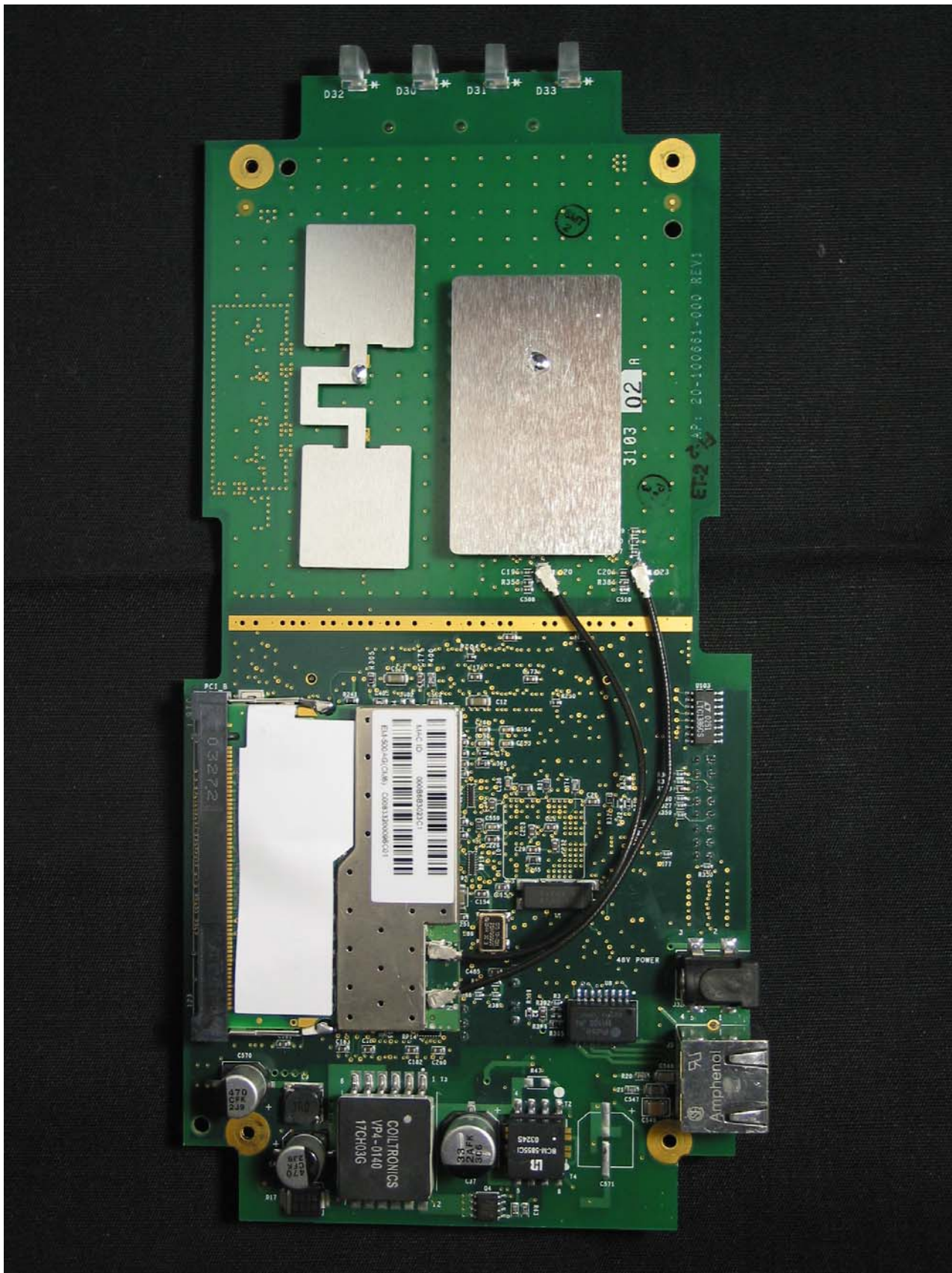
Model 1200 B/G accesspoint, B side, internal
