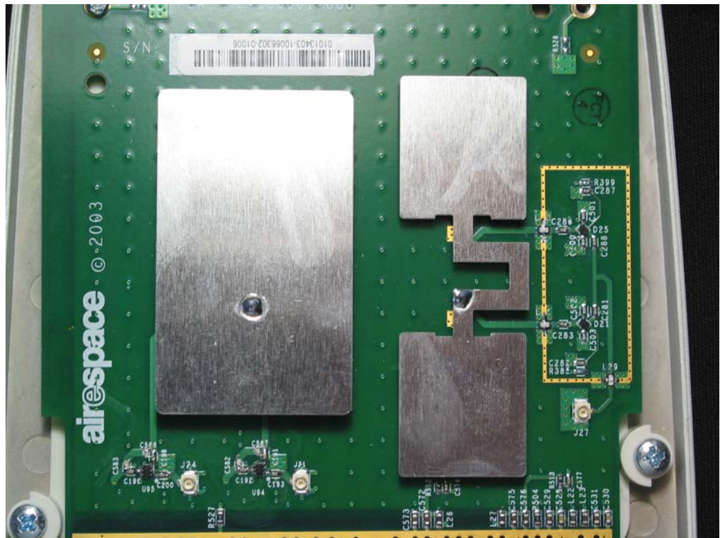
Model 1200 B/G access point. A side antennas Left (2.4 GHz) Right (5 GHz)
