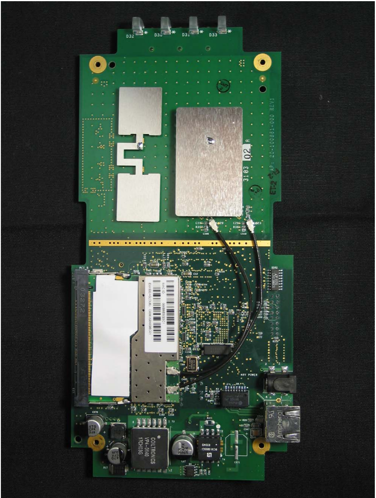
Model 1200 A/B/G accesspoint, B side, internal
