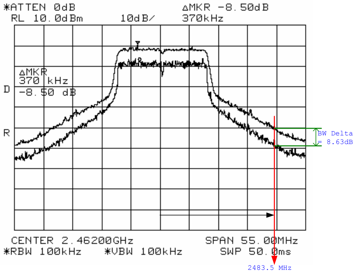
2483.5 MHz BW delta measurement
