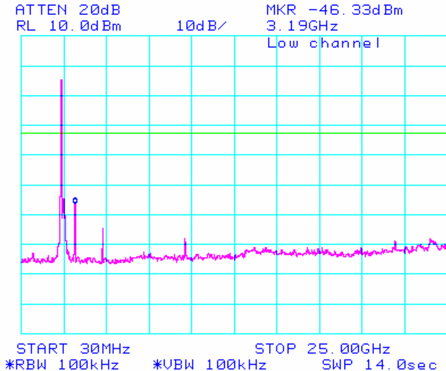
OBE Emissions, Transmit on Channel 1 (2412MHz)
