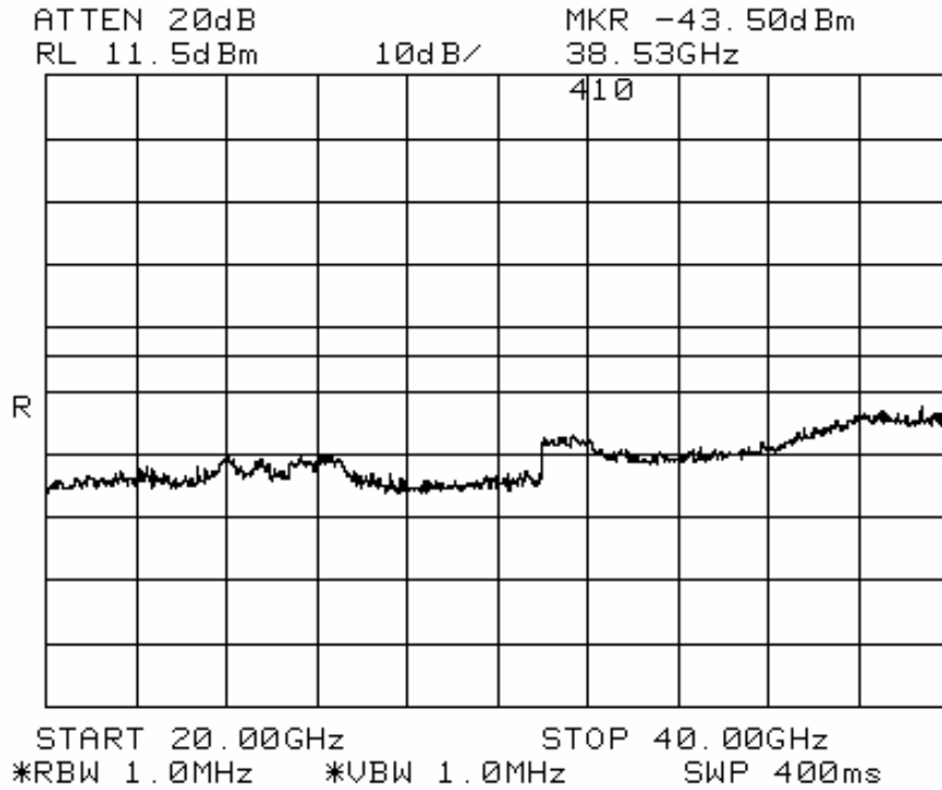
Lower UNII band(s) emissions plots UUT Transmitting on 5.32 GHz
