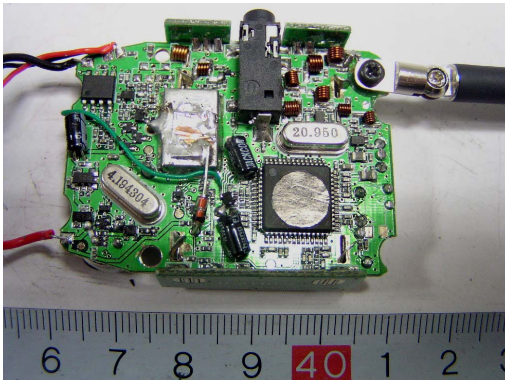
EUT-PCB View (2)
