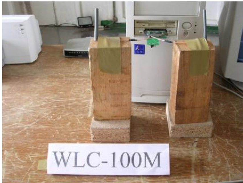
Photo 2: Spurious Emission Set-up
