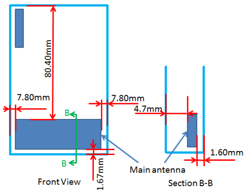
Distance Between Device Edges and Faces and Main Antenna
