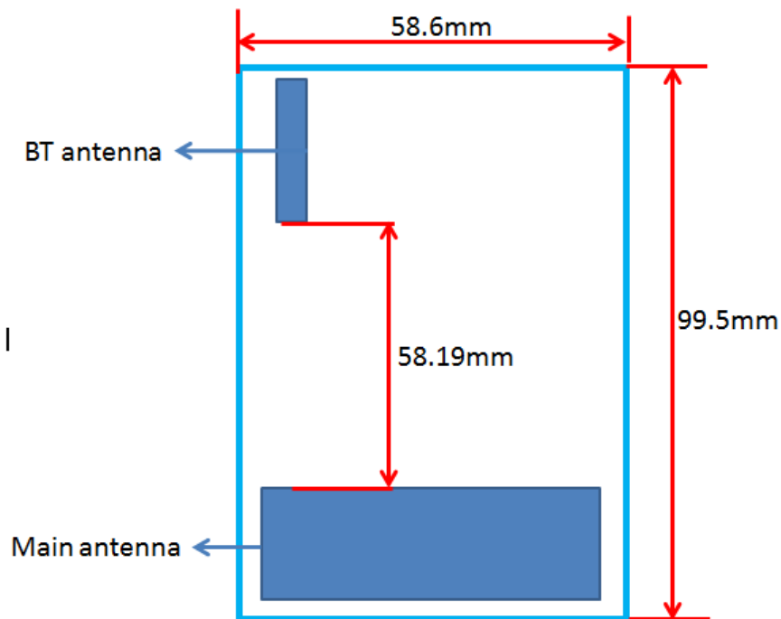
Phone Outside Dimension and Distance Between Main Antenna and BT Antenna
