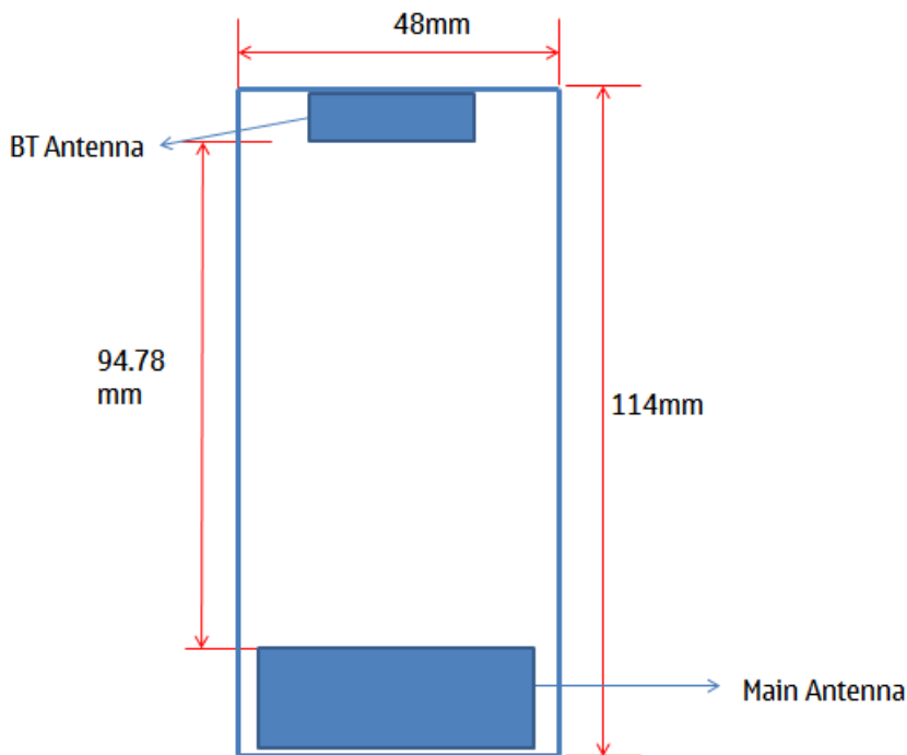
Phone Dimension and Distance Between Main antenna and BT Antenna
