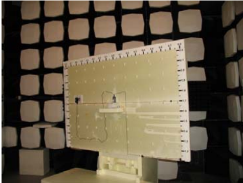
Picture 1. FCC Part 15C Radiated emissions
