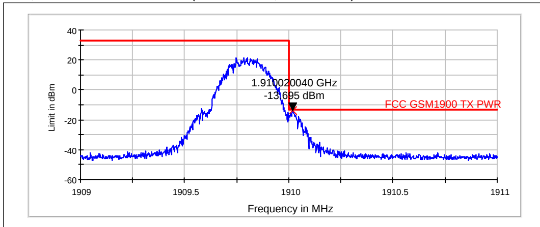
GSM, channel 810 / 1909.8 MHz (Peak detector, RBW: 3 kHz)
