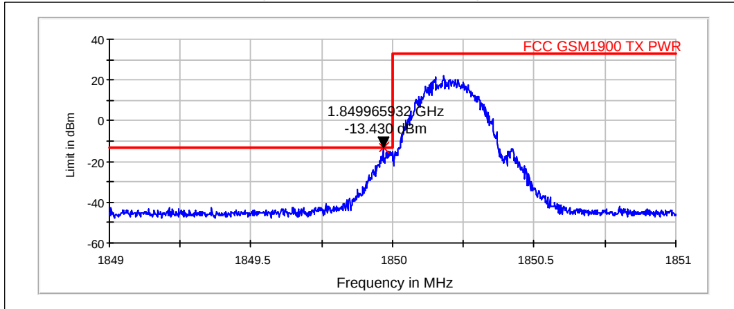
GSM, channel 512 / 1850.2 MHz (Peak detector, RBW: 3 kHz)
