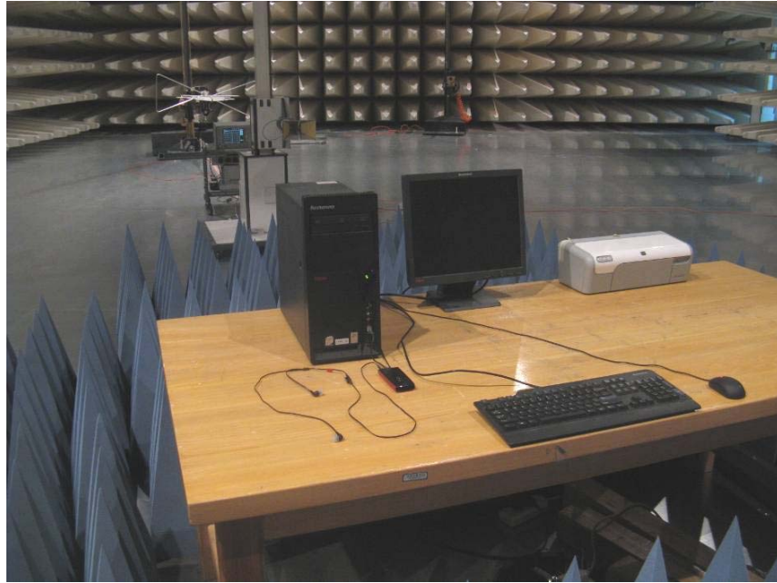
Radiated Emission - Data Transferring (Above 1GHz)
