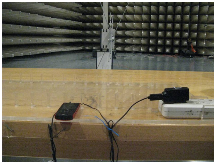
Radiated Emission- FM & GPS
