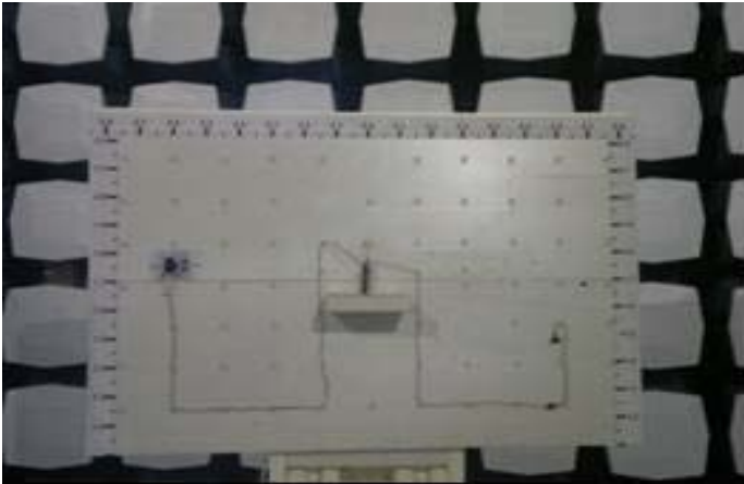
Picture 1. FCC Part 15C Radiated emissions
